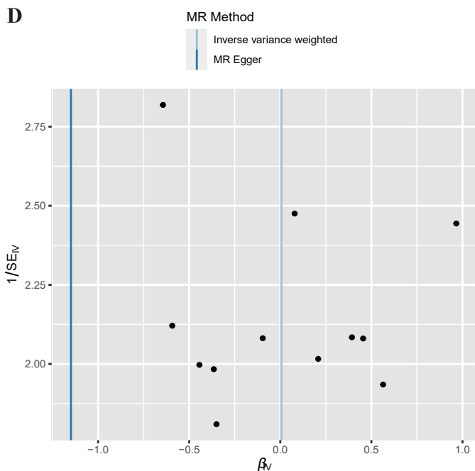
Supplementary Figure 6. Forest plot (A), sensitivity analysis (B), scatter plot (C), and funnel plot (D) of the causal effect of Paraprevotella on UIA risk.
