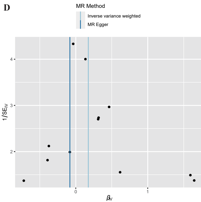
Supplementary Figure 7. Forest plot (A), sensitivity analysis (B), scatter plot (C), and funnel plot (D) of the causal effect of the whole gut microbiome on UIA risk.
