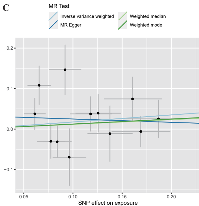
Supplementary Figure 7. Forest plot (A), sensitivity analysis (B), scatter plot (C), and funnel plot (D) of the causal effect of the whole gut microbiome on UIA risk.
