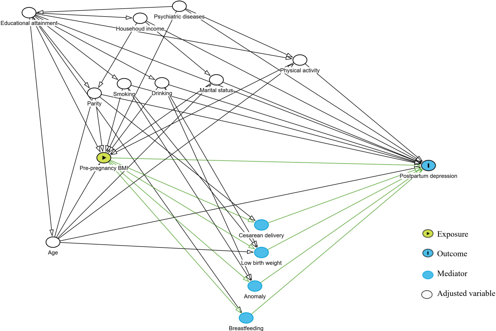
Additional file 1 Directed Acyclic Graph illustrating the assumed causal and mediation relationships.
