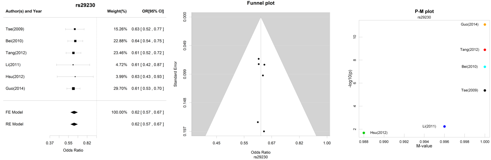
Supplementary Figure S2 Forest plots, funnel plots and P-M plots for NPC association (part III). a) rs9260734; b) rs2517713; c) rs3129055; d) rs29232; e) rs29230. Left: Forest plots of ORs with 95% CIs for polymorphisms and NPC susceptibility. Middle and Right: funnel plots and P–M plots represent the publication bias test.
