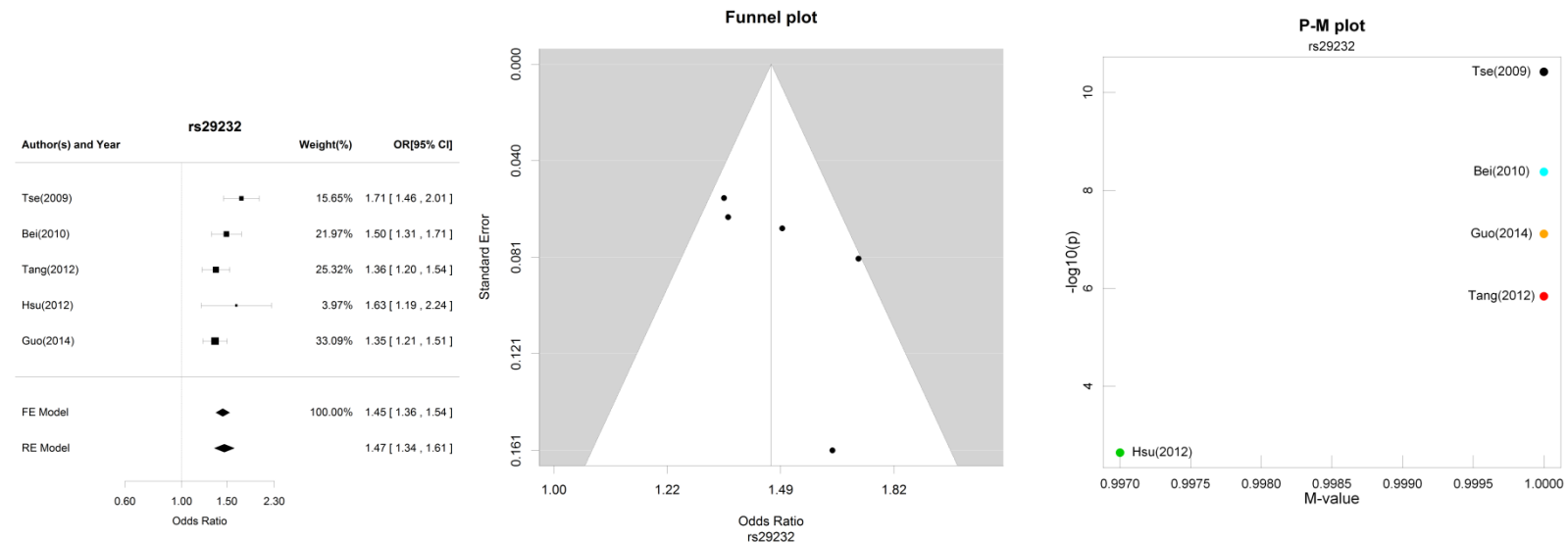
Supplementary Figure S2 Forest plots, funnel plots and P-M plots for NPC association (part II).
