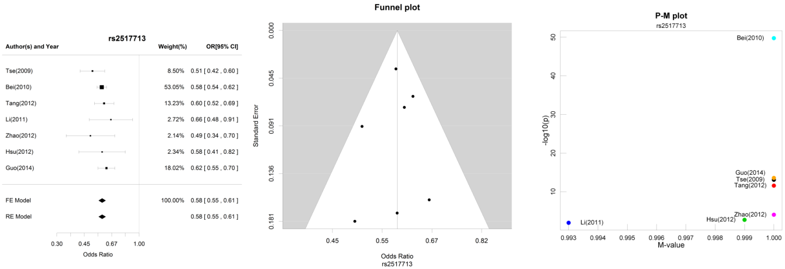
Supplementary Figure S2 Forest plots, funnel plots and P-M plots for NPC association (part I)
