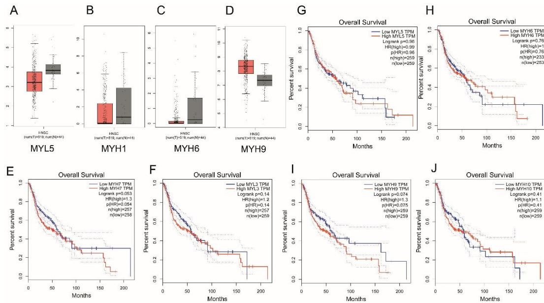
Figure S1 Gene chip analysis of myosin genes in head and neck squamous cell carcinoma and expression level and survival time analysis in TCGA database.
