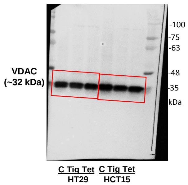
Western blot of loading control (VDAC)
