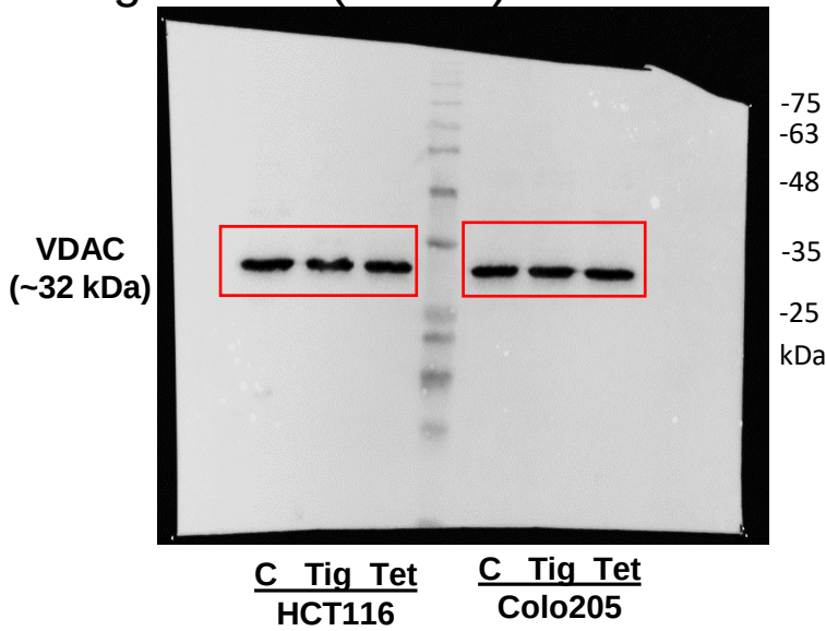
Western blot of loading control (VDAC)
