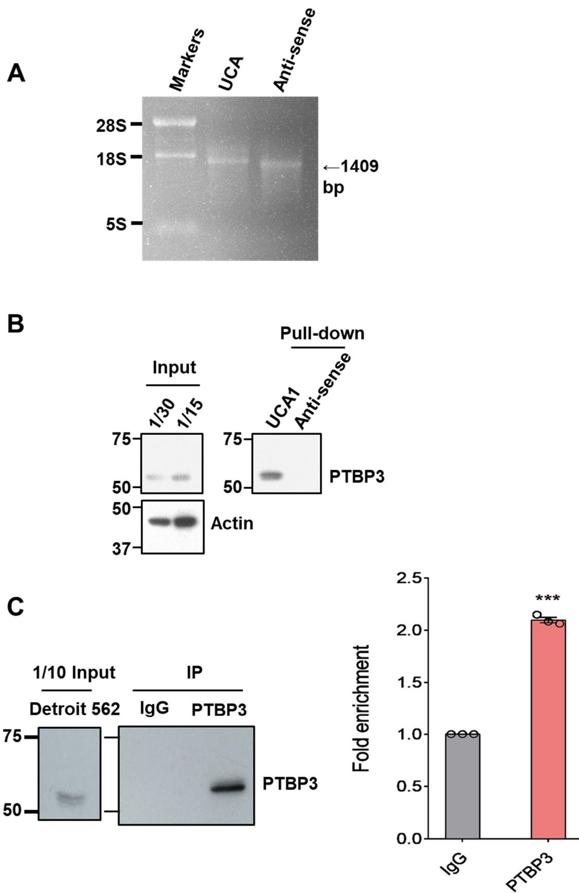
Fig. S4. PTBP3 is identified as a UCA1 -interacting partner.
