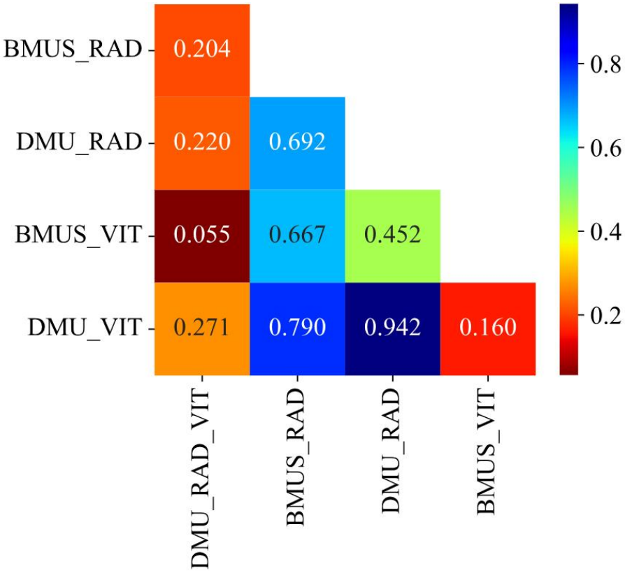
Cohort internal test Delong
