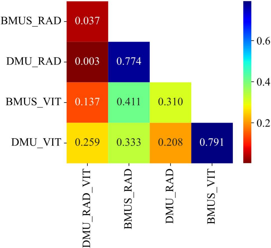
Cohort external test Delong
