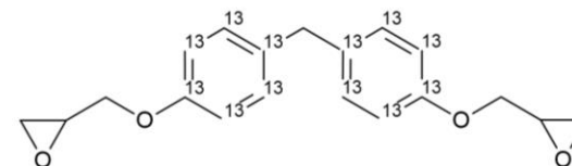
Bisphenol F diglycidyl ether (RING- 13 C 12 ) (BFDGE- 13 C 12 )
