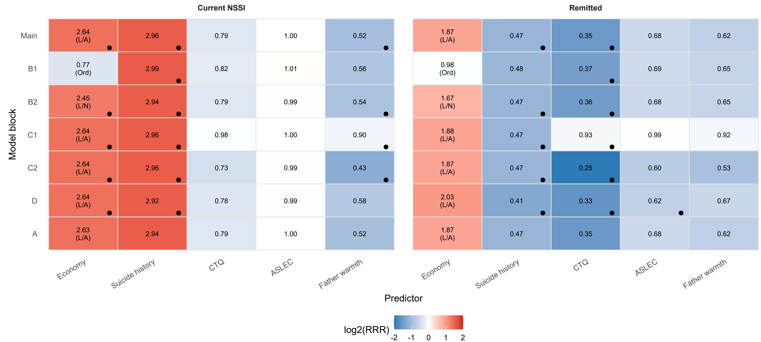
Figure S2. Robustness heatmap (including block A, re-baselined)
