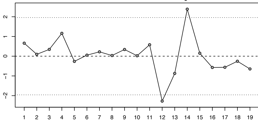
rstudent
