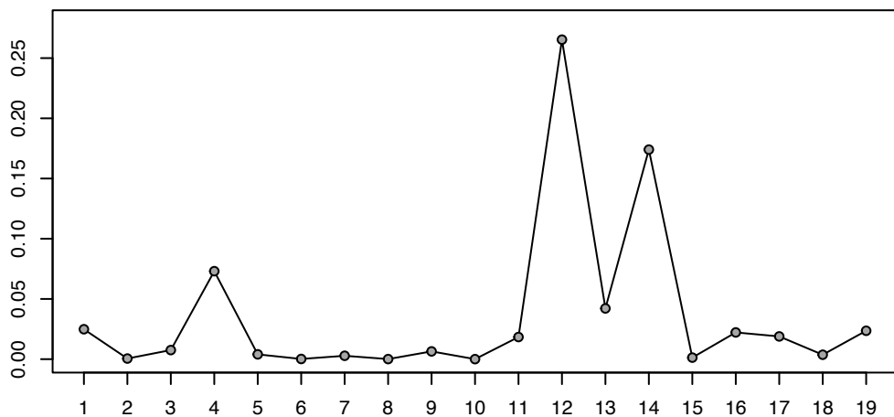
cook.d
