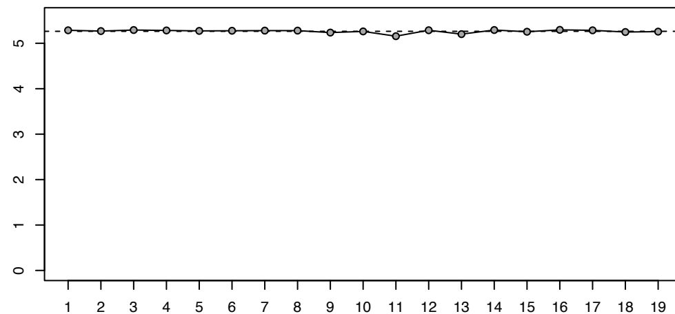
weight
