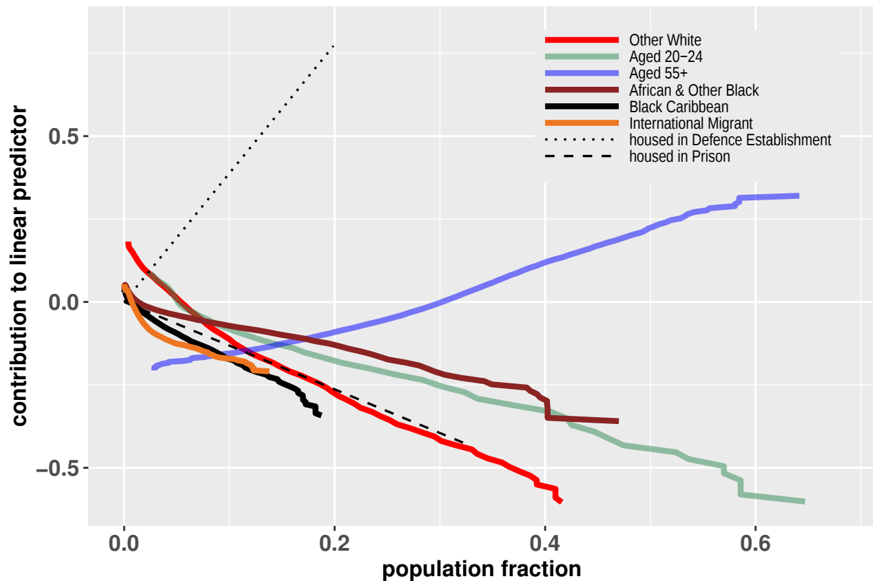
M1 (1st Primary) contributions of some key univariate smoothers
