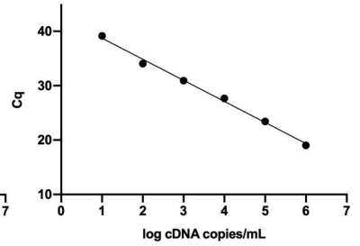
Tbp
