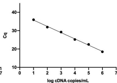
Tbp
