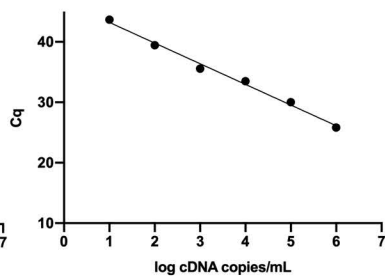
Runx-2
