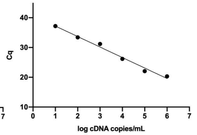
Runx-2
