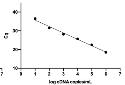
Tgf- \beta_3
