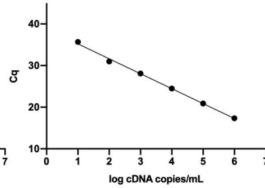
Sdha
