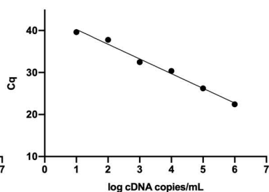
Tgf- \beta_3
