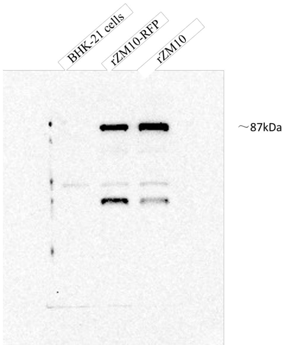
Figure S2-B1. Western blotting result of NDV HN protein expression
