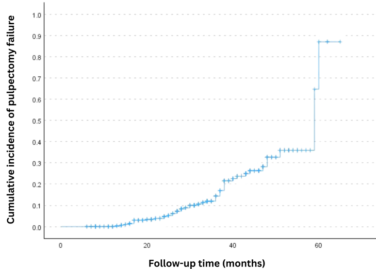
a. Unweighted Kaplan–Meier Estimate Plotted as Cumulative Incidence
