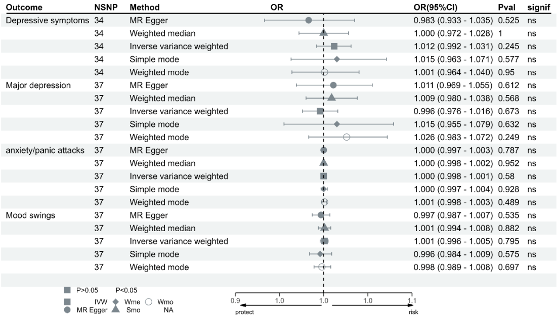
Supplementary Figure S2 The effect of genetically determined UFs on psychological factors using UVMR.
