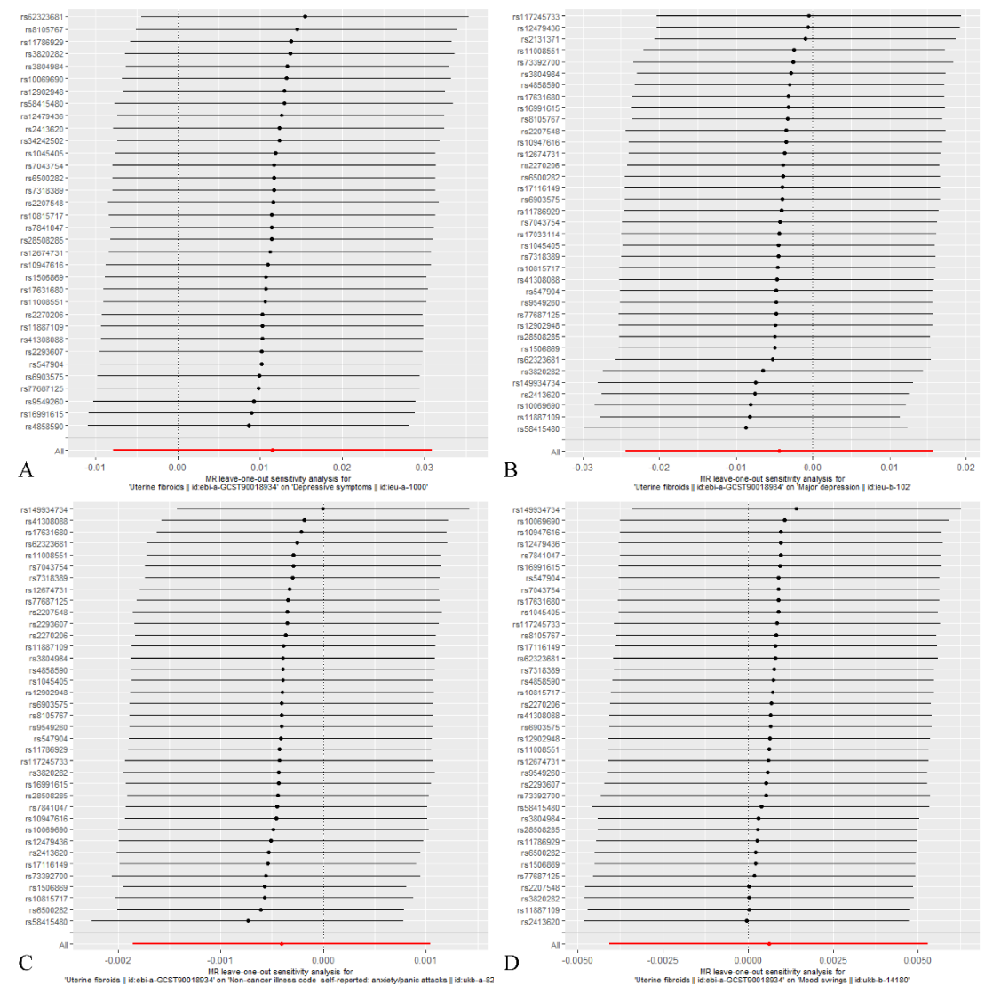
Supplementary Figure S4 The leave-one-out plots for MR analyses of the correlation between UFs and psychological factors. (A) depressive symptoms; (B) MDD; (C) anxiety or panic attacks; (D) mood swings.
