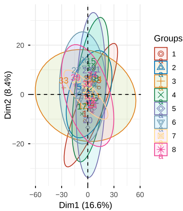
Batch effect PC 1 & 2
