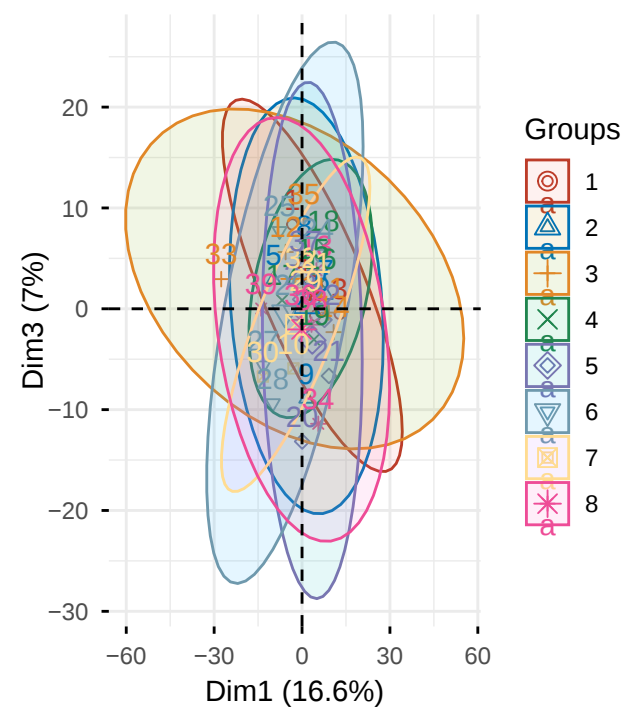
Batch effect PC 1 & 3
