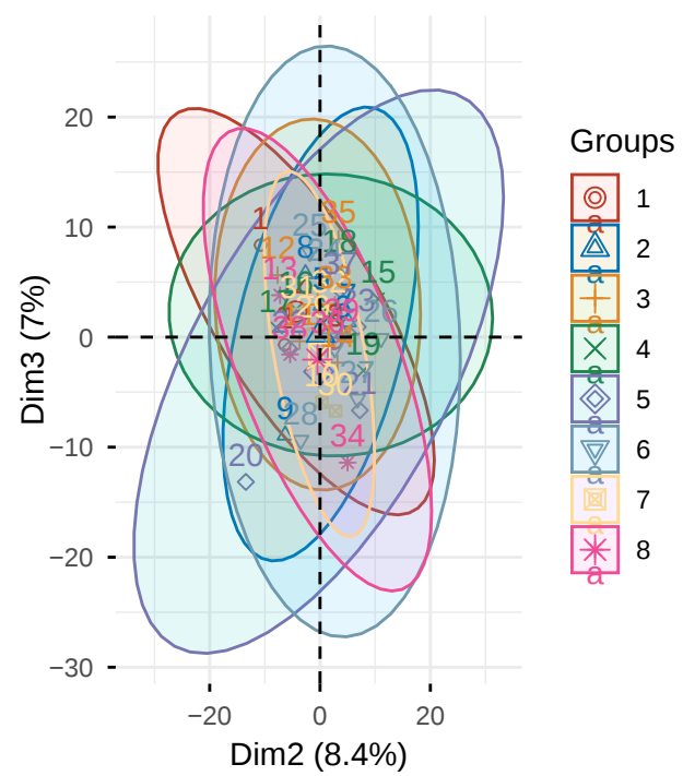
Batch effect PC 2 & 3
