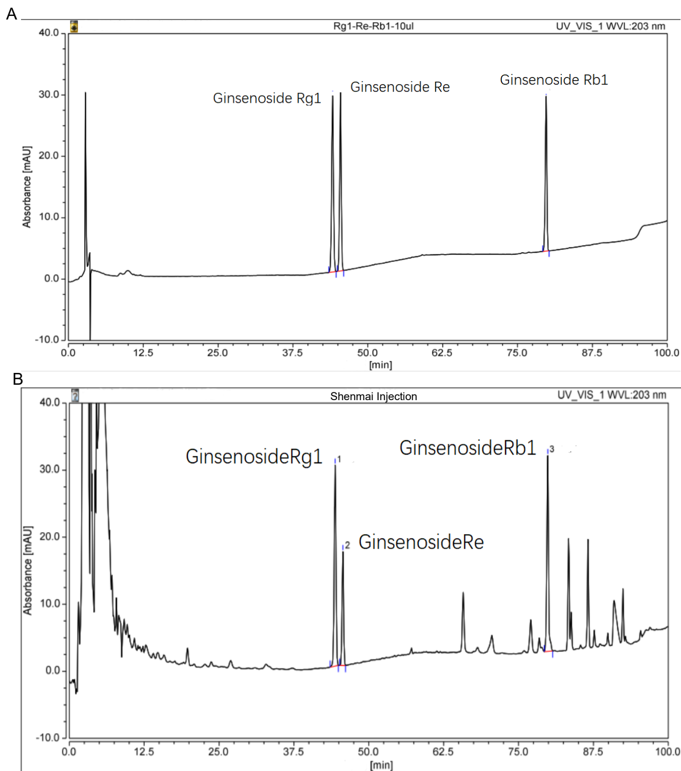
Figure S1. (A) The chromatogram of Ginsenoside Rg1、Re、Rb1 reference solution. (B) The chromatogram of Shenmai injection test solution.
