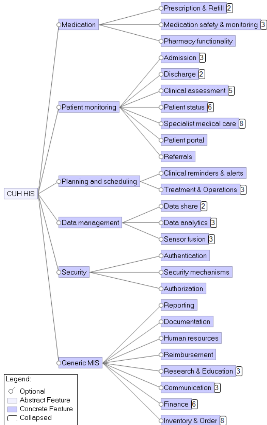
Figure 1: Downsized version of the feature model for the Chiba University Hospital based on Jahn et al. [59]. Numbers on the right hand side of the features represent the number of sub-features shown.
