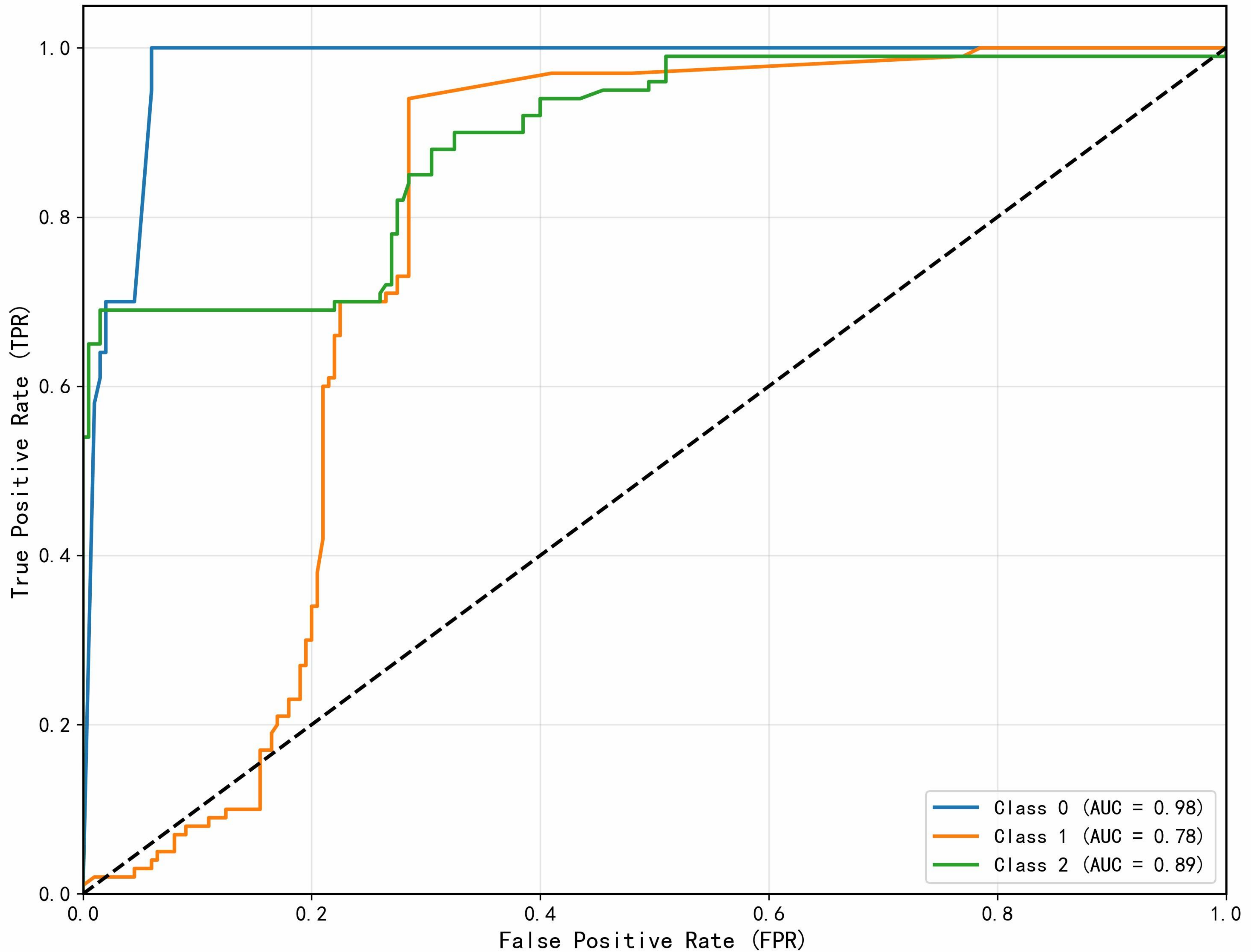
XGBoost Multiclass ROC Curve
