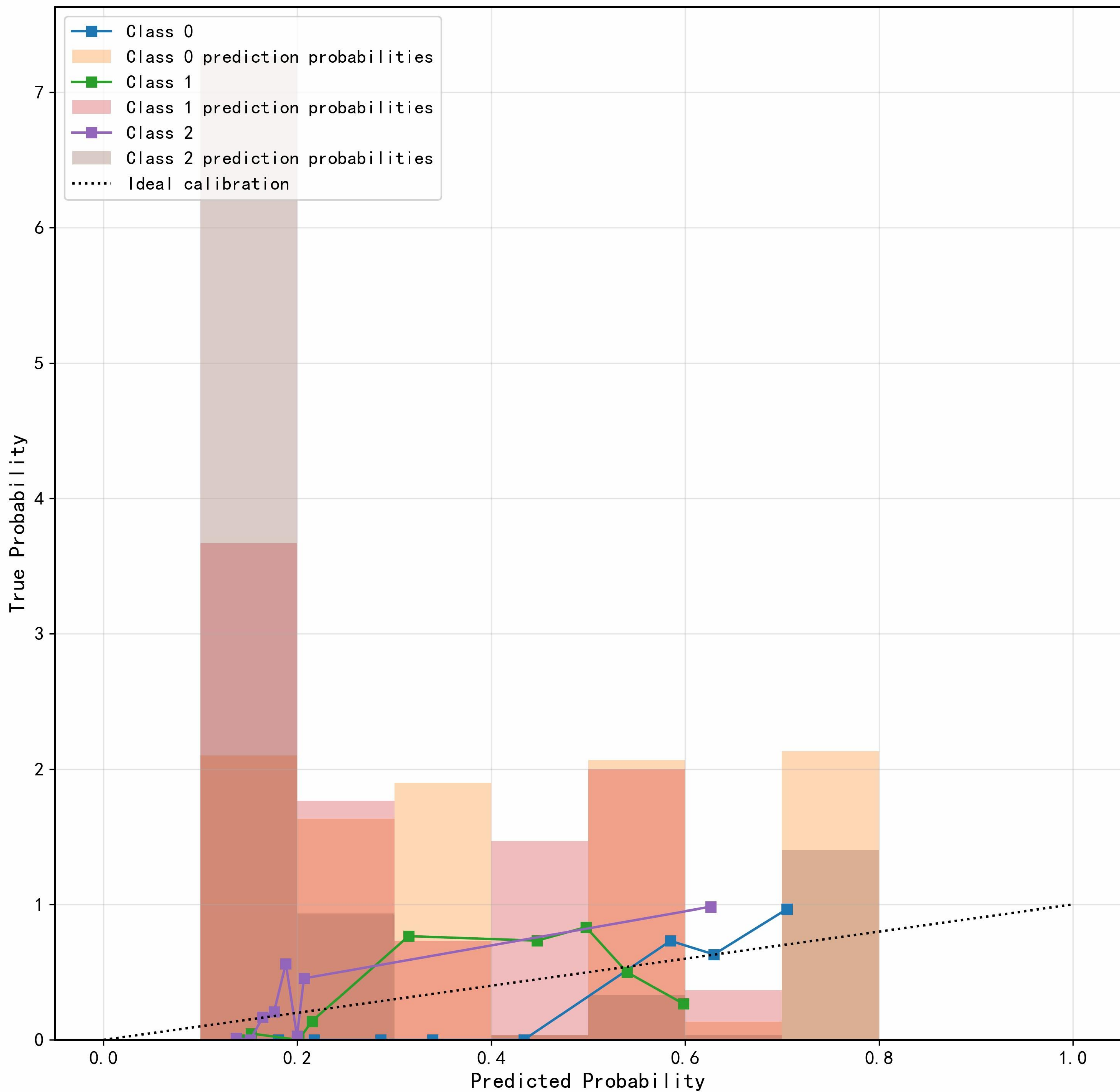
XGBoost Calibration Curve
