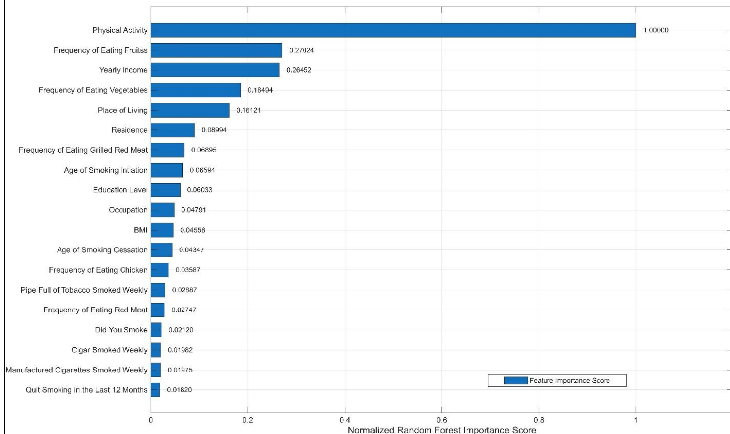
Selected Features Ranked by Random Forest
