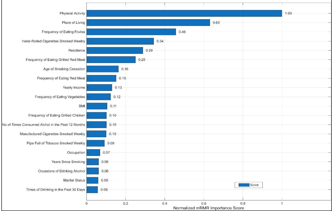
Selected Features Ranked by mRMR
