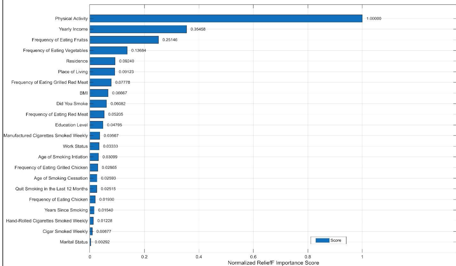
Selected Features Ranked by ReliefF
