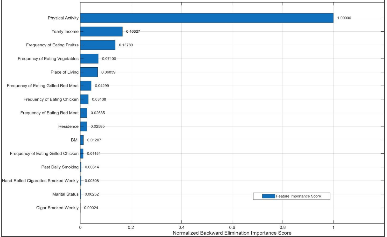
Selected Features Ranked by Backward Elimination + Permutation Importance
