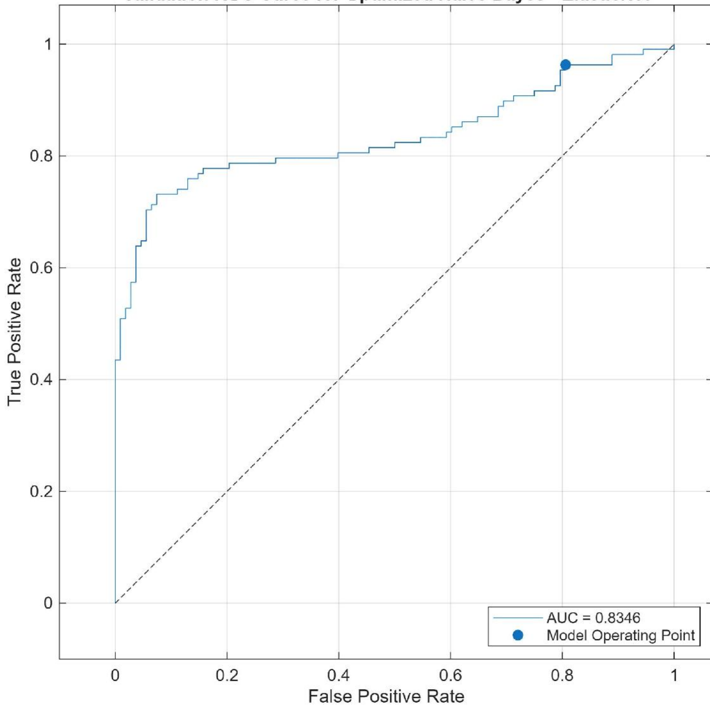
Validation ROC Curve for Optimized Naive Bayes - ElasticNet
