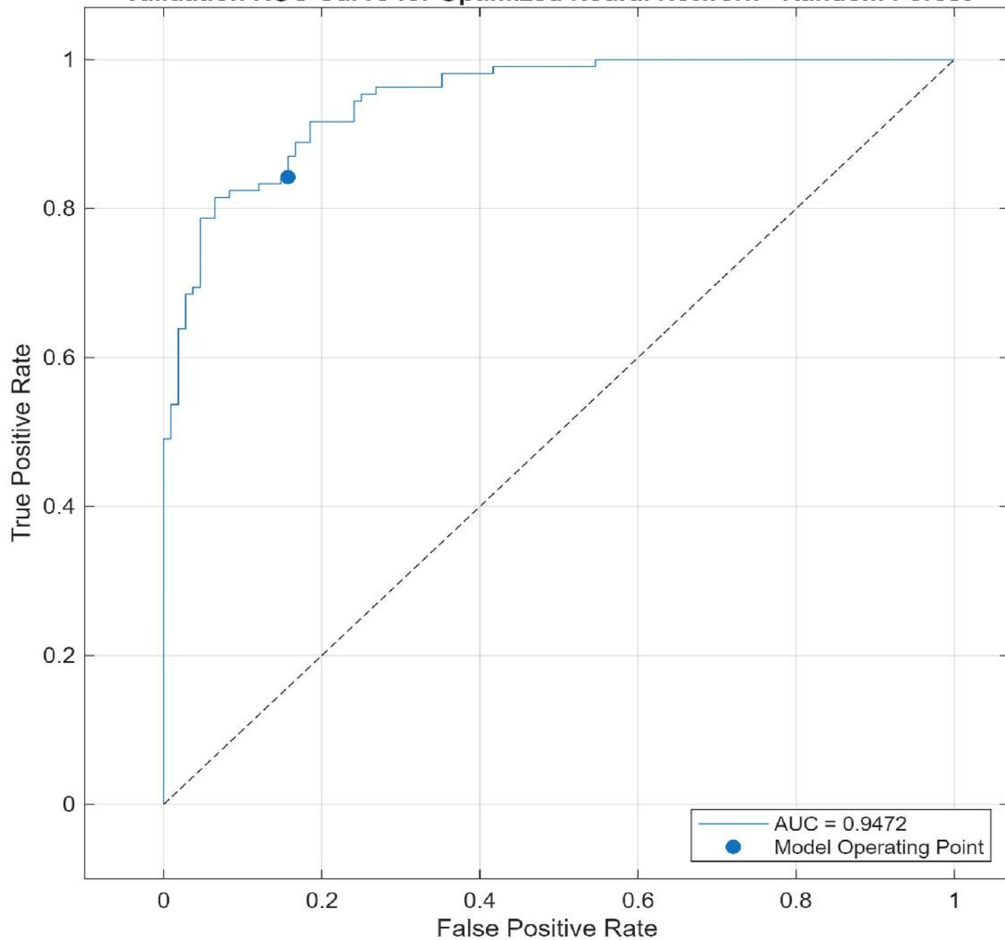
Validation ROC Curve for Optimized Neural Network - Random Forest
