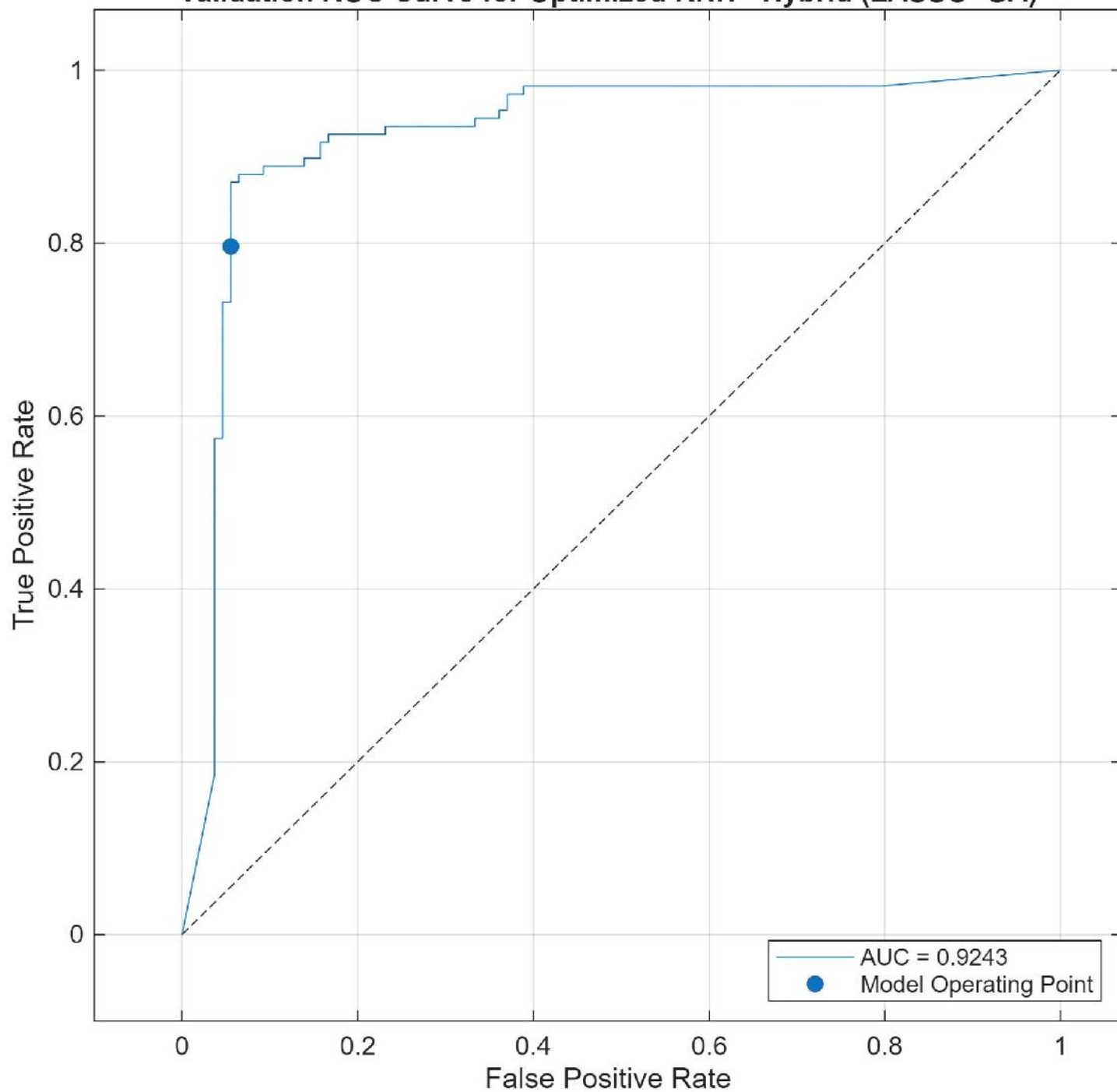
Validation ROC Curve for Optimized KNN - Hybrid (LASSO+GA)
