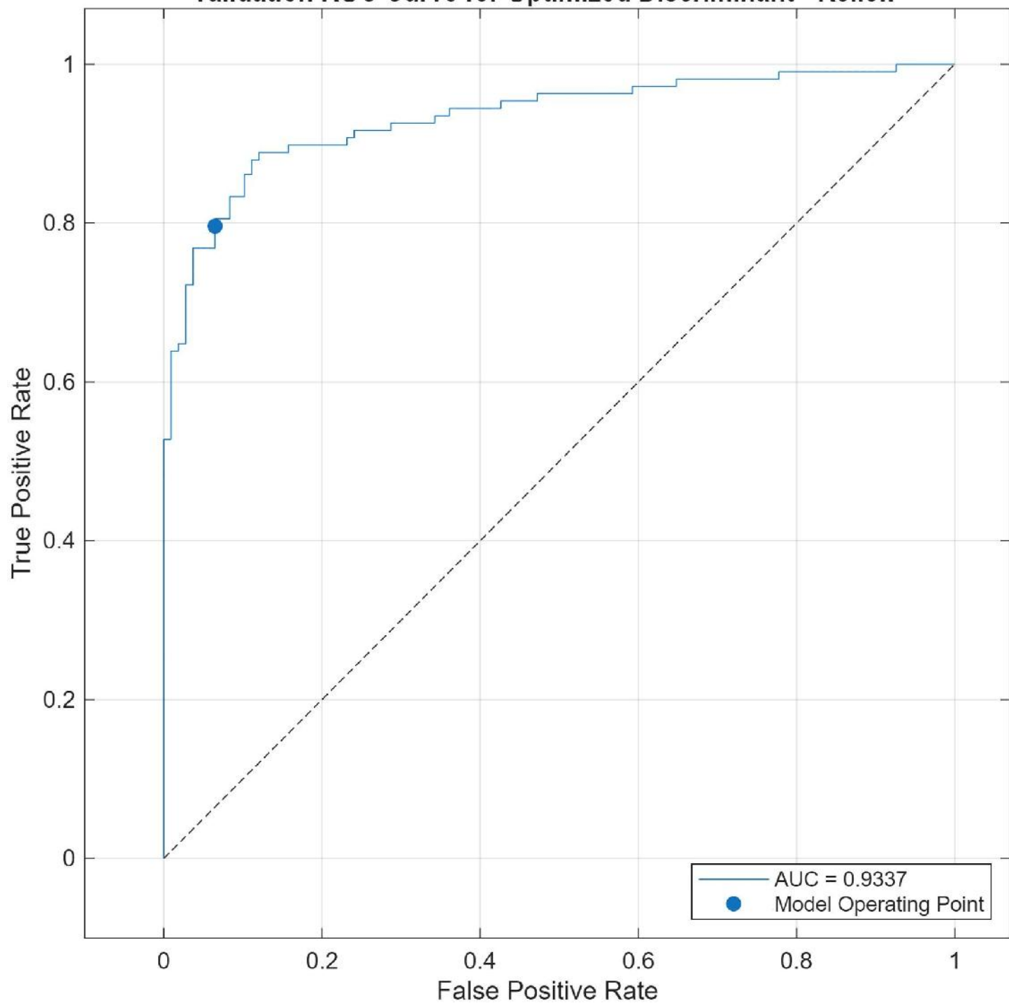
Validation ROC Curve for Optimized Discriminant - ReliefF
