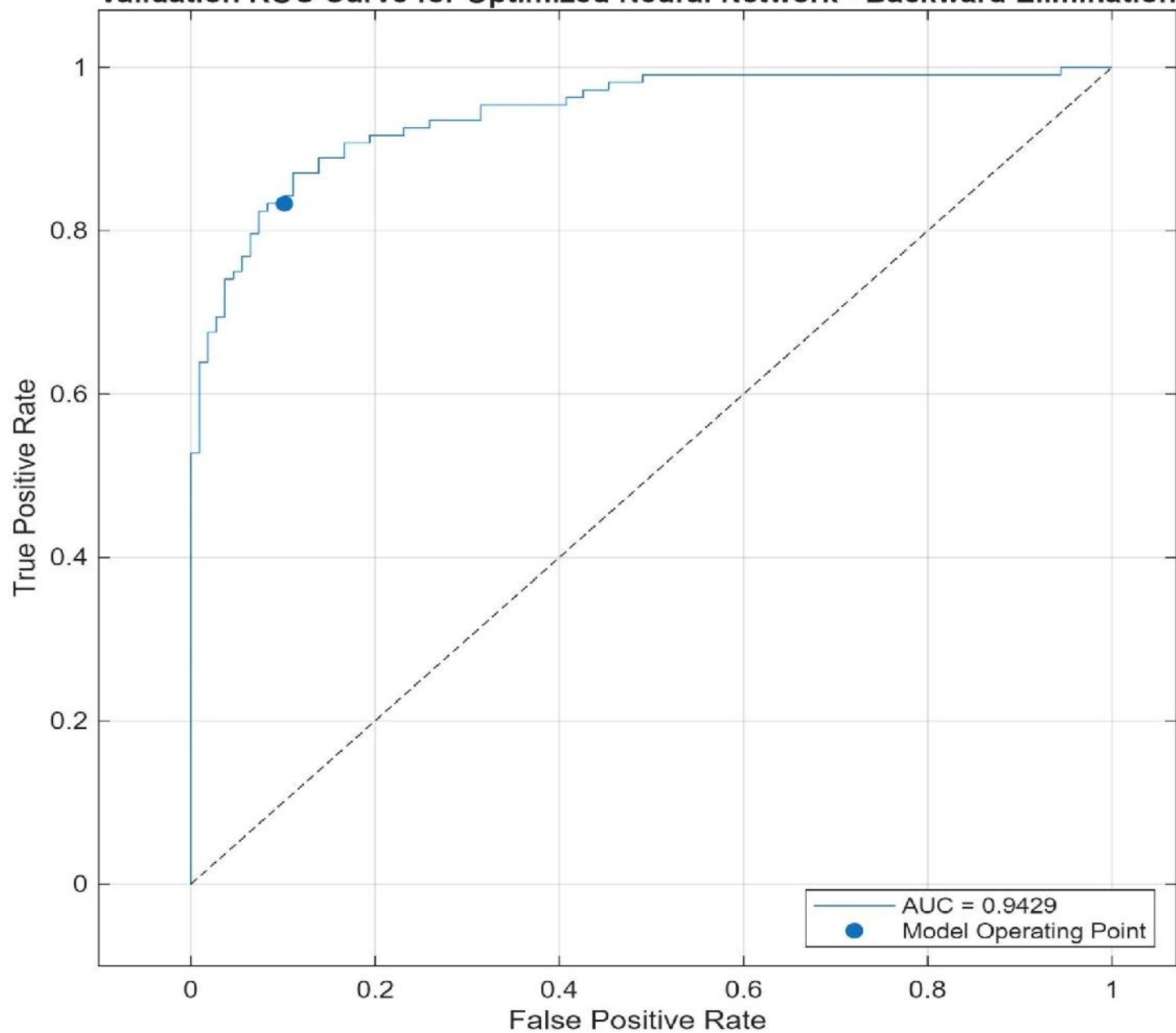
Validation ROC Curve for Optimized Neural Network - Backward Elimination
