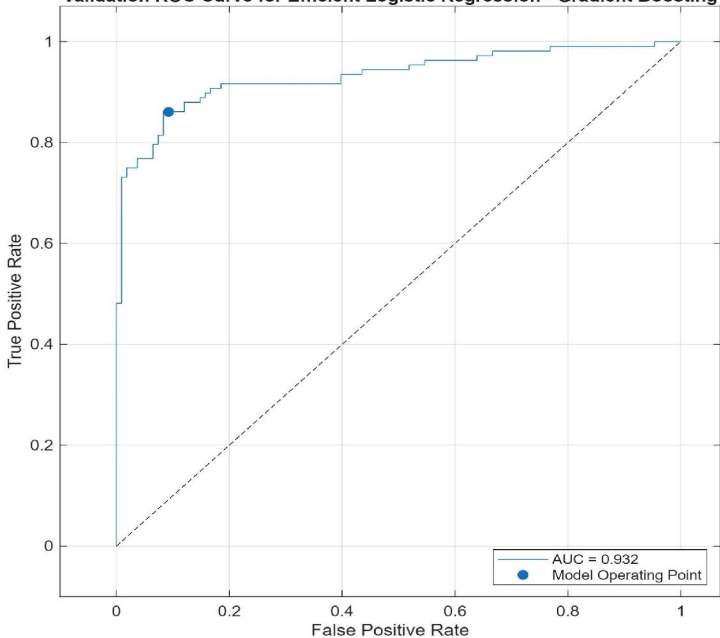
Validation ROC Curve for Efficient Logistic Regression - Gradient Boosting
