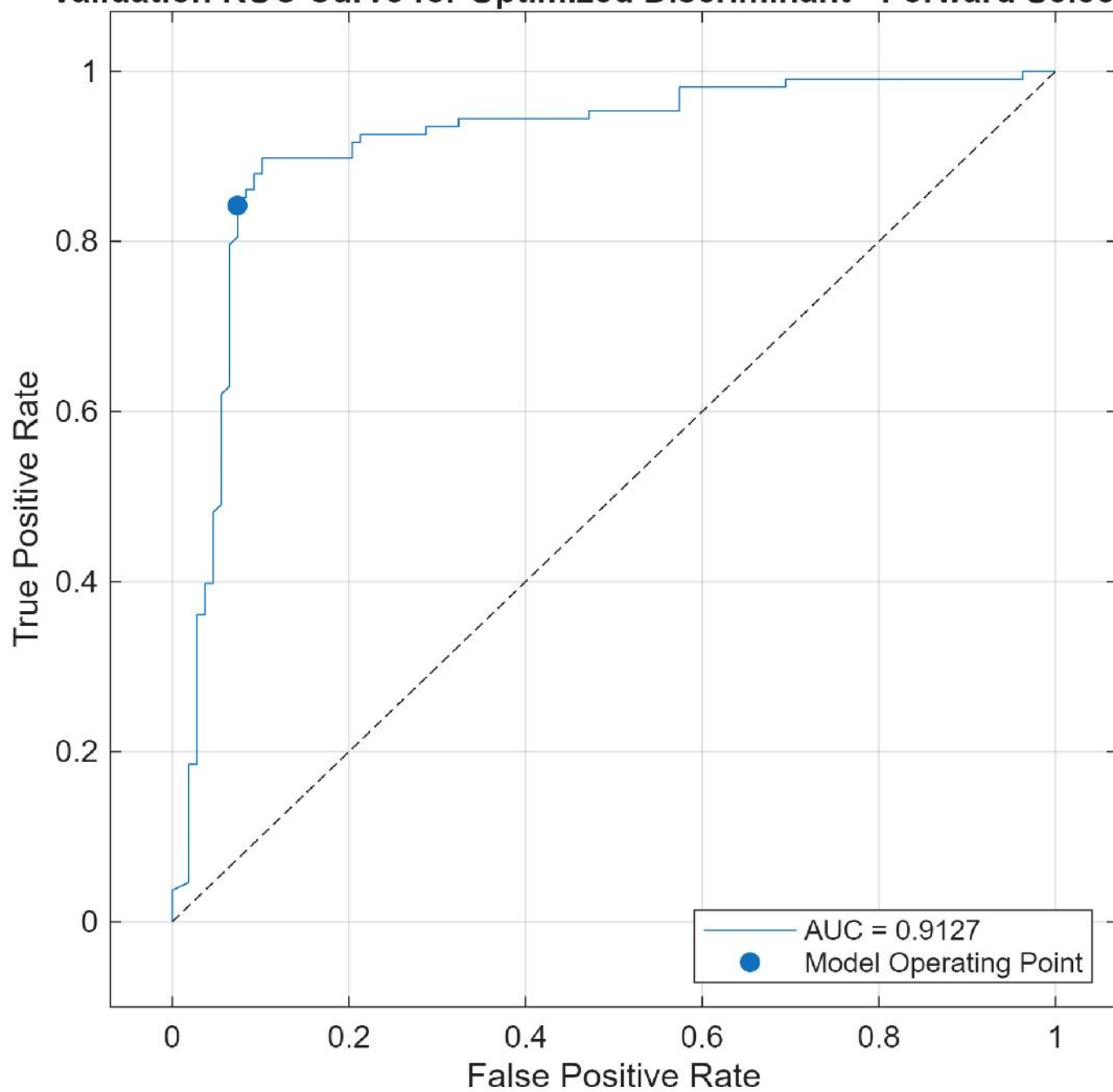
Validation ROC Curve for Optimized Discriminant - Forward Selection
