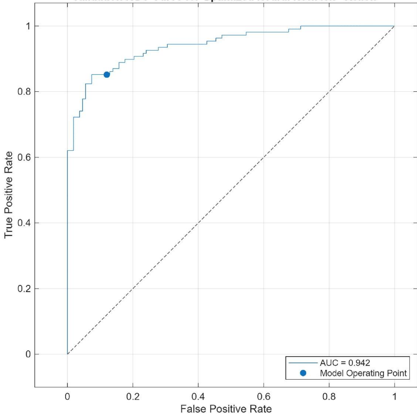
Validation ROC Curve for Optimized Neural Network - ReliefF
