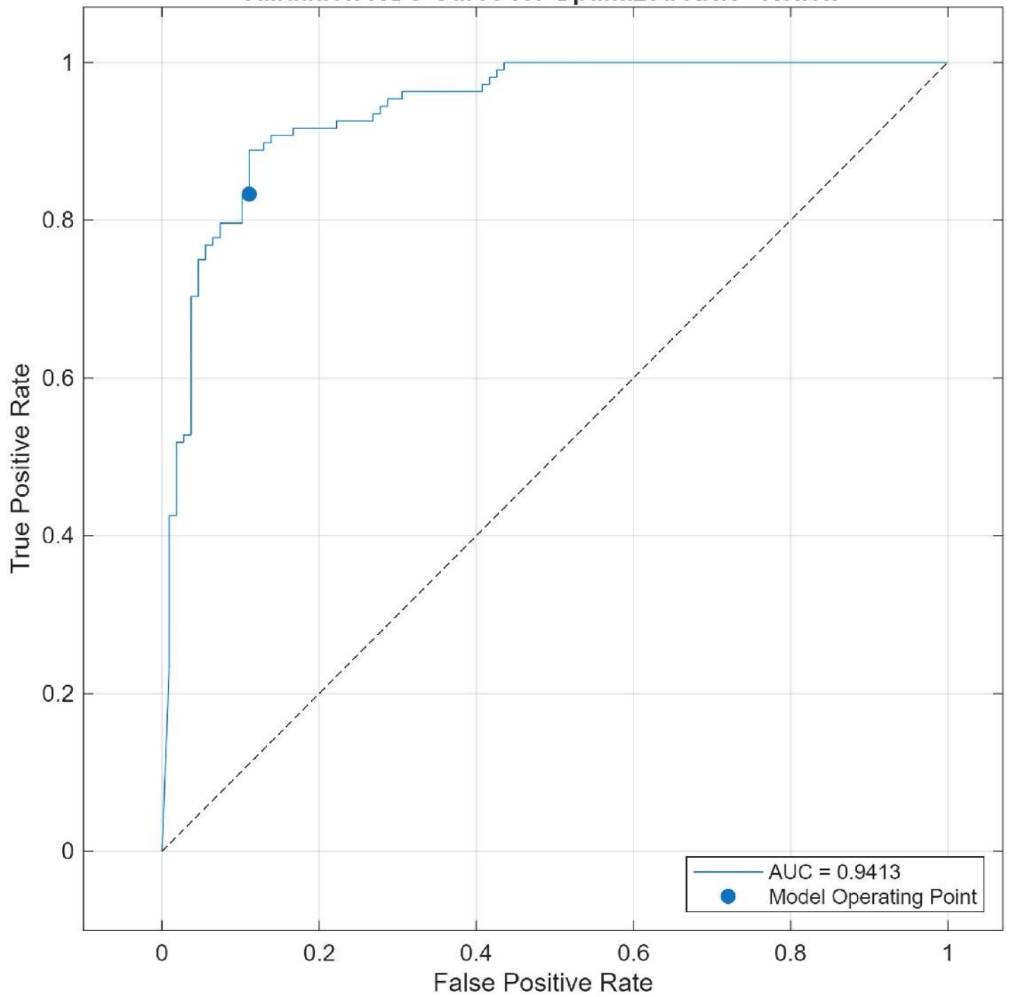
Validation ROC Curve for Optimized KNN - ReliefF
