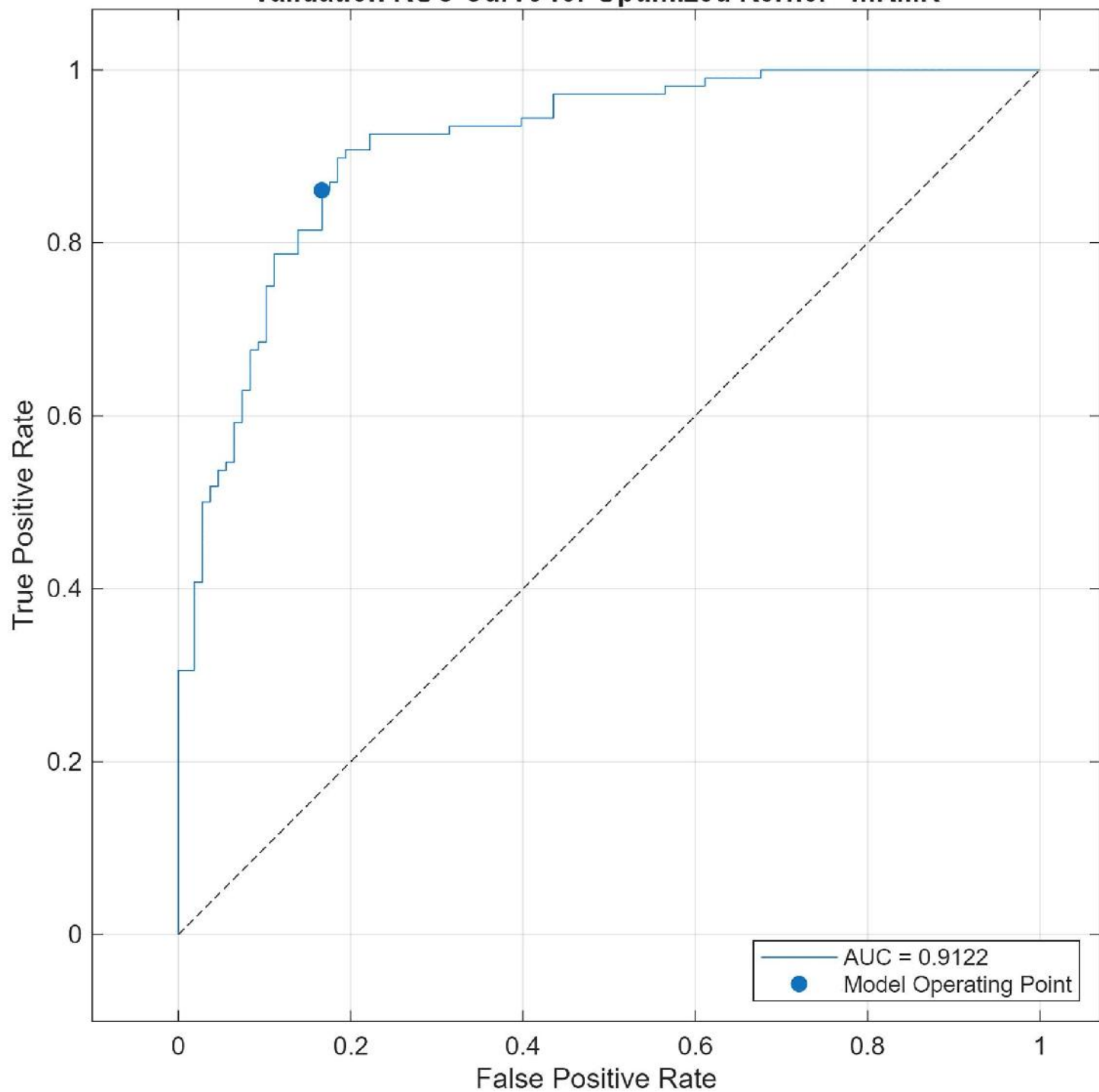
Validation ROC Curve for Optimized Kernel - mRMR
