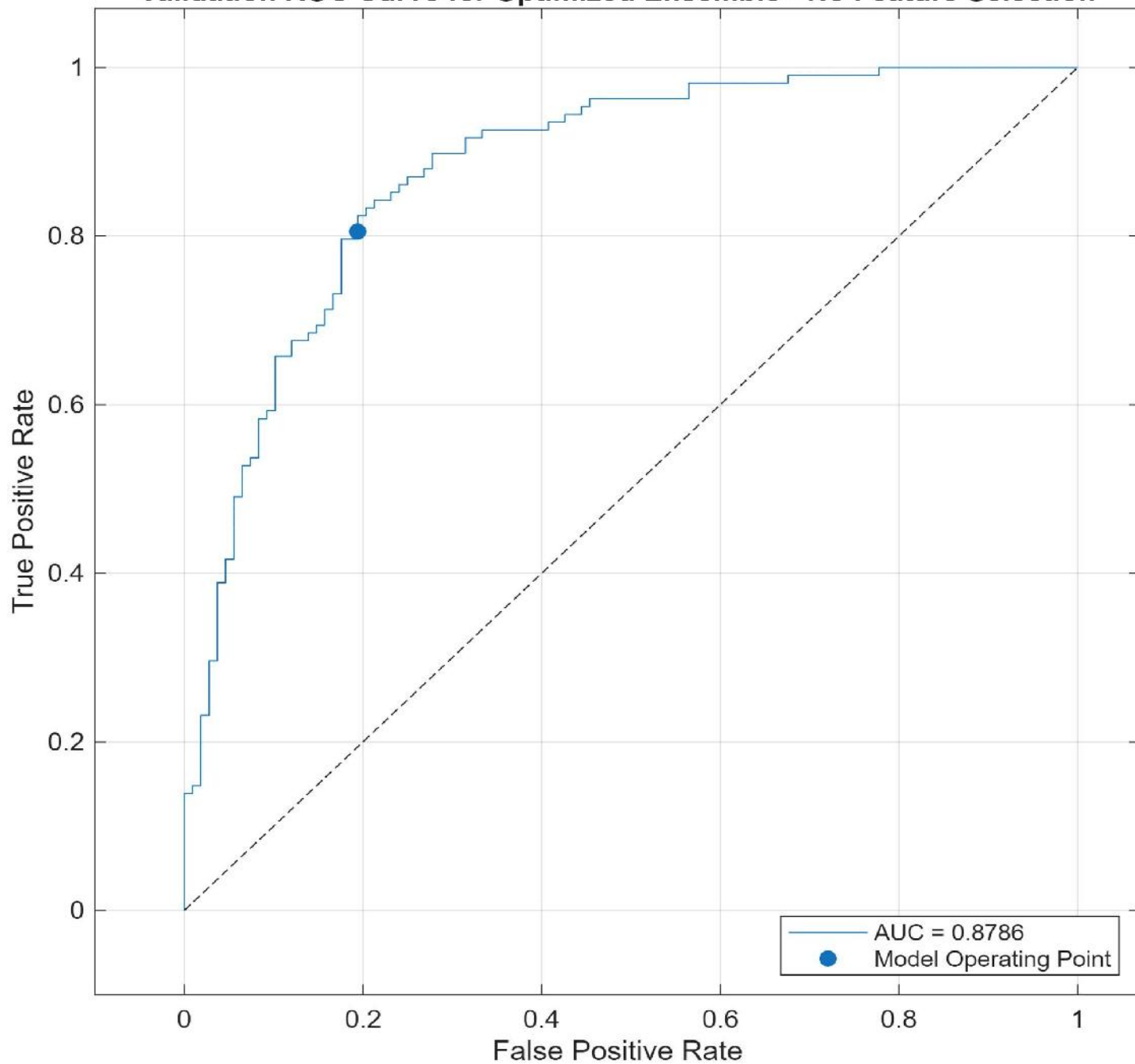
Validation ROC Curve for Optimized Ensemble - No Feature Selection
