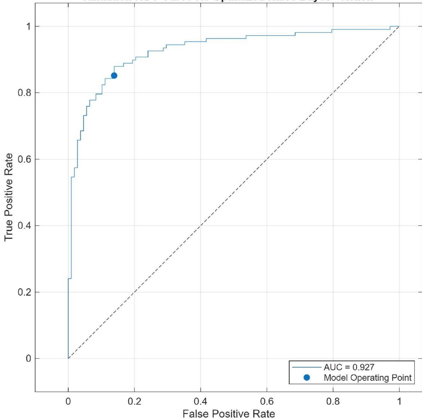
Validation ROC Curve for Optimized Naive Bayes - ReliefF
