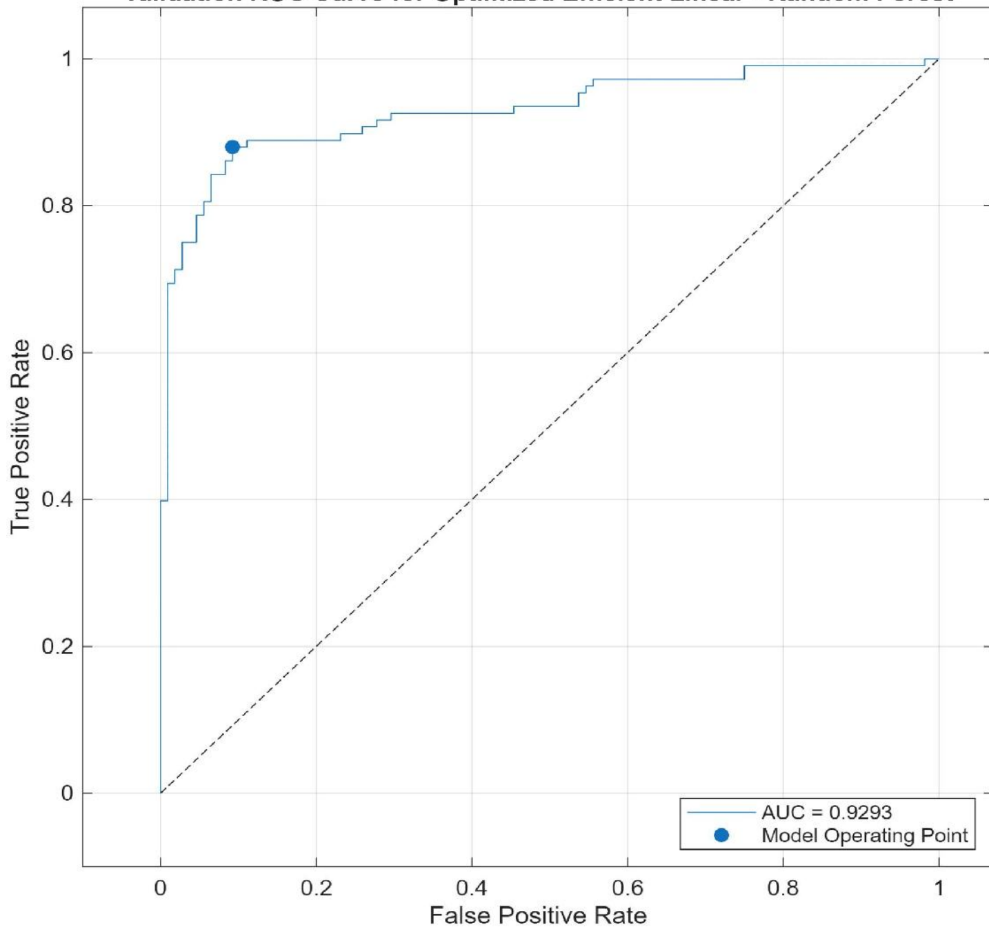
Validation ROC Curve for Optimized Efficient Linear - Random Forest
