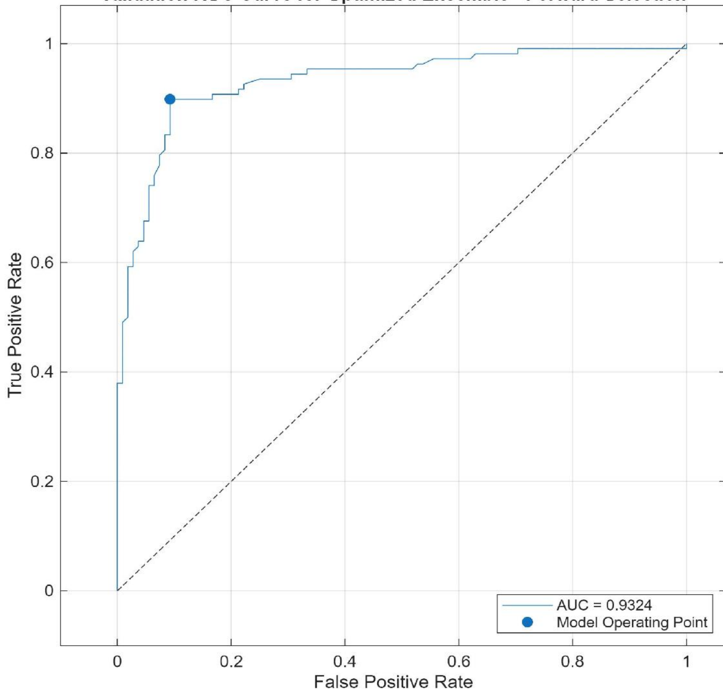
Validation ROC Curve for Optimized Ensemble - Forward Selection
