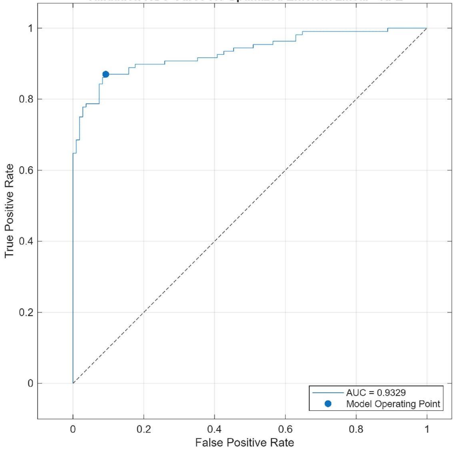
Validation ROC Curve for Optimized Efficient Linear - RFE
