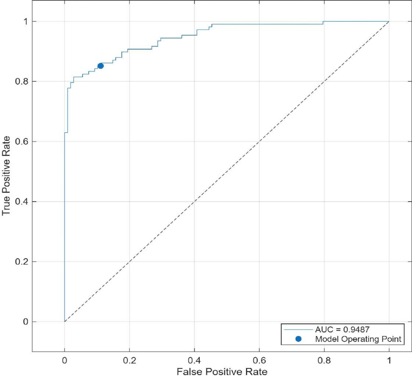
Validation ROC Curve for Optimized Neural Network - Gradient Boosting
