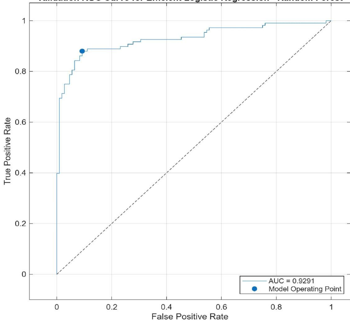
Validation ROC Curve for Efficient Logistic Regression - Random Forest
