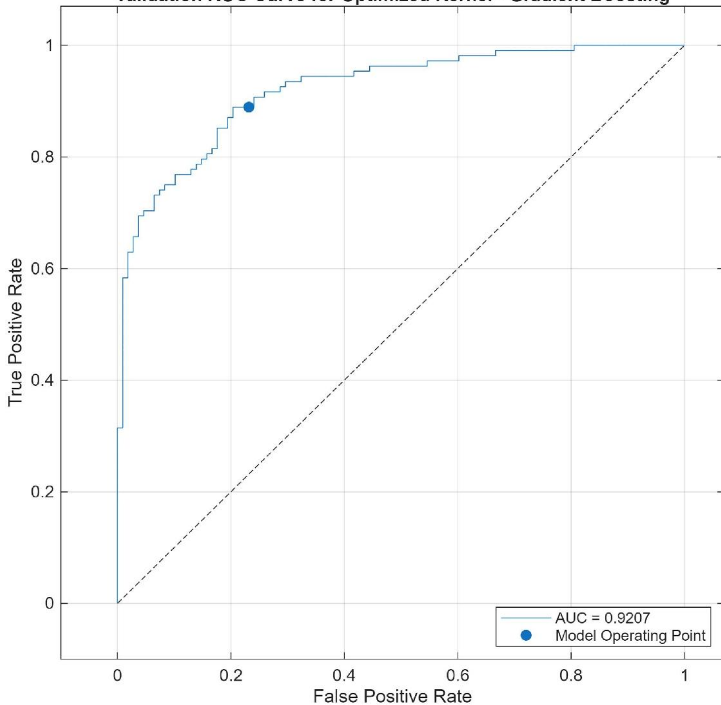
Validation ROC Curve for Optimized Kernel - Gradient Boosting
