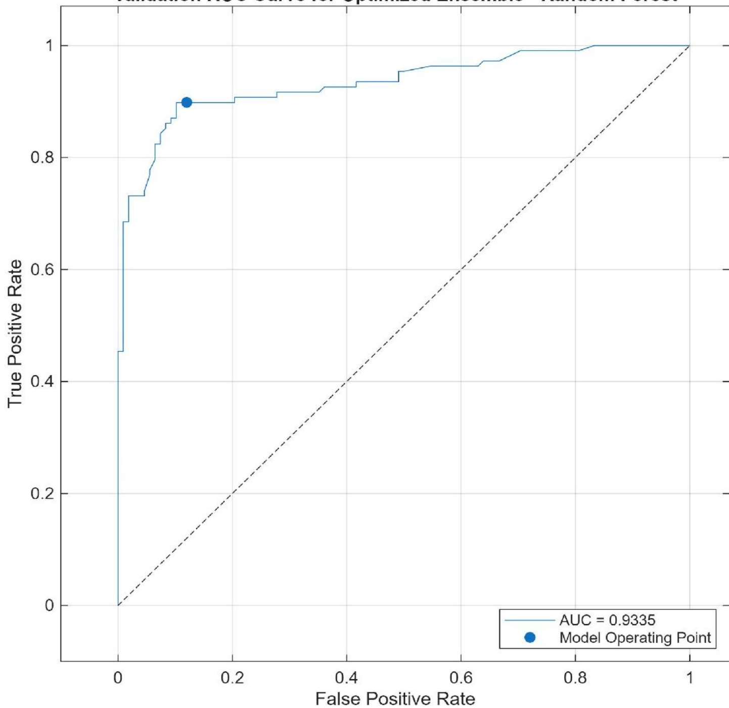
Validation ROC Curve for Optimized Ensemble - Random Forest
