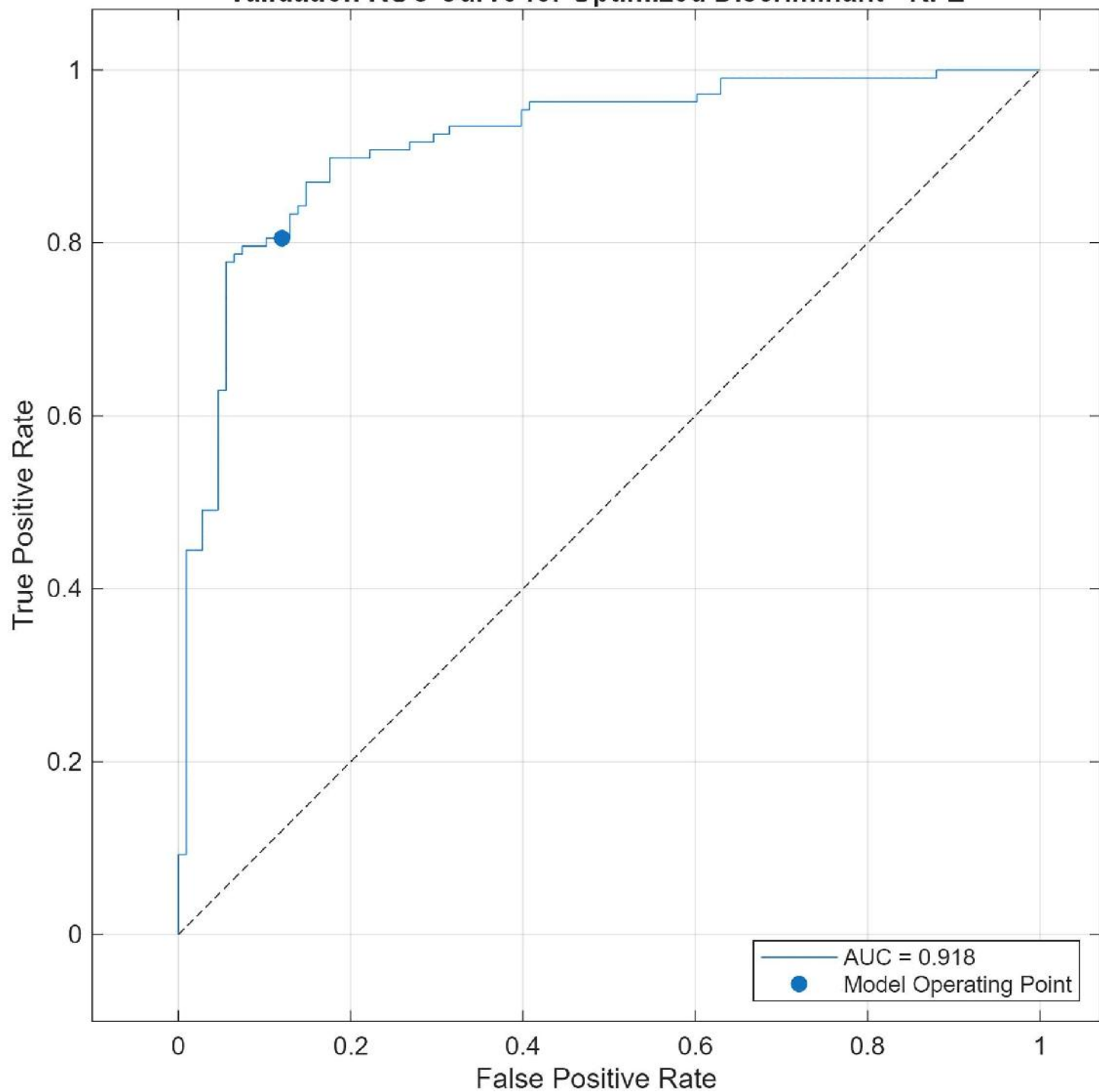
Validation ROC Curve for Optimized Discriminant - RFE
