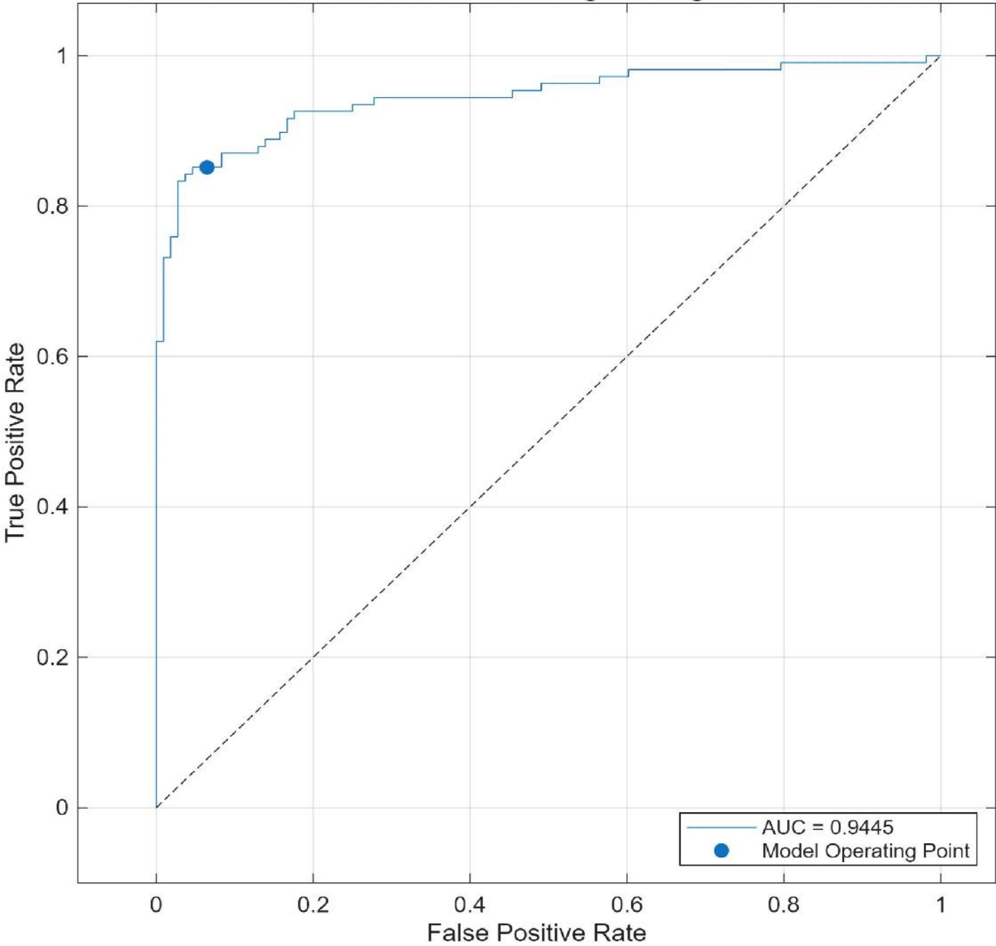
Validation ROC Curve for Efficient Logistic Regression - ElasticNet
