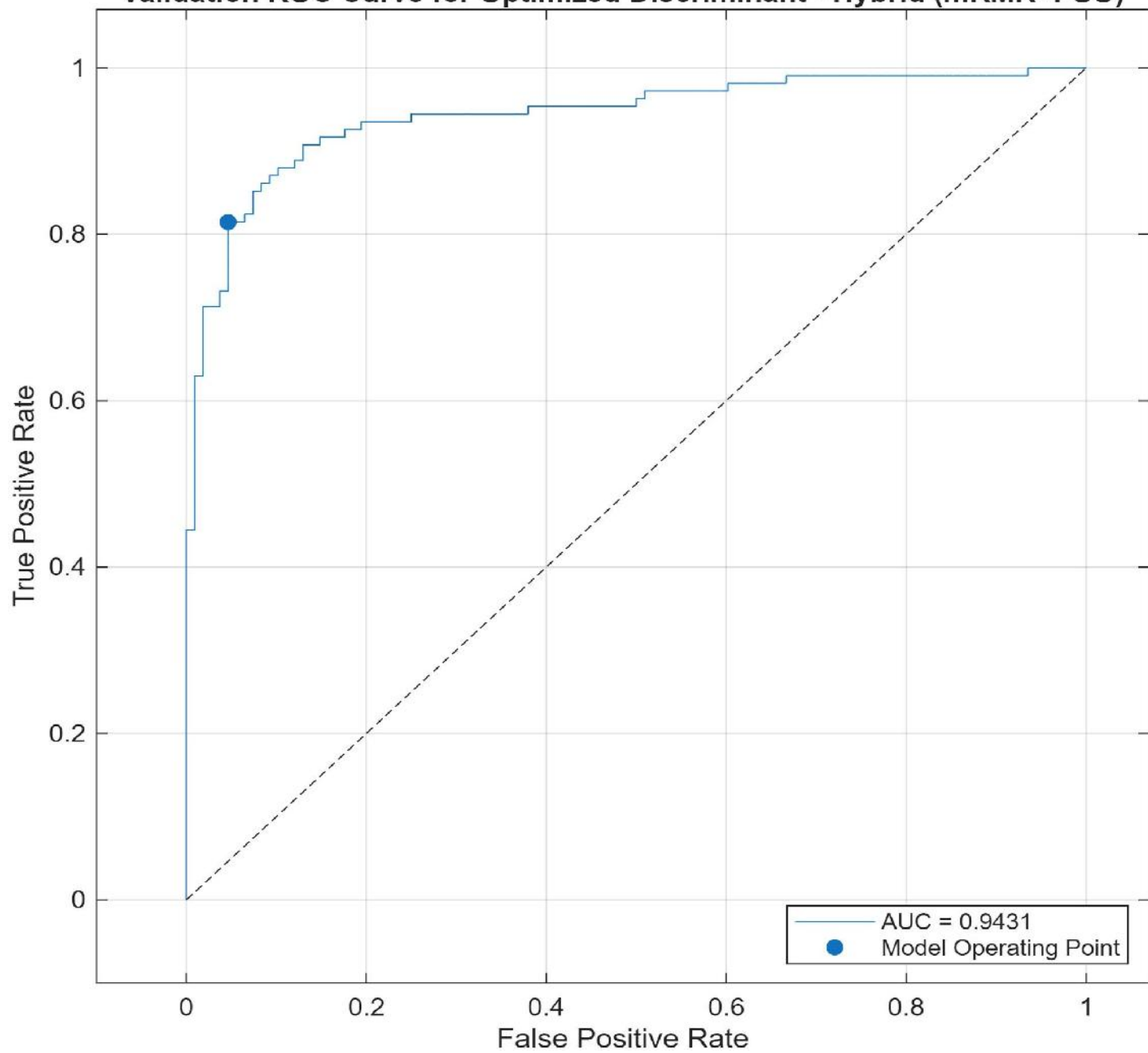
Validation ROC Curve for Optimized Discriminant - Hybrid (mRMR+PSO)
