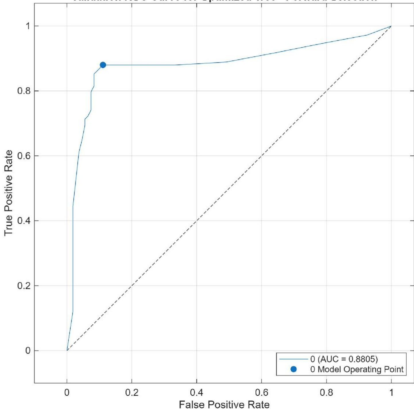
Validation ROC Curve for Optimized Tree - Forward Selection
