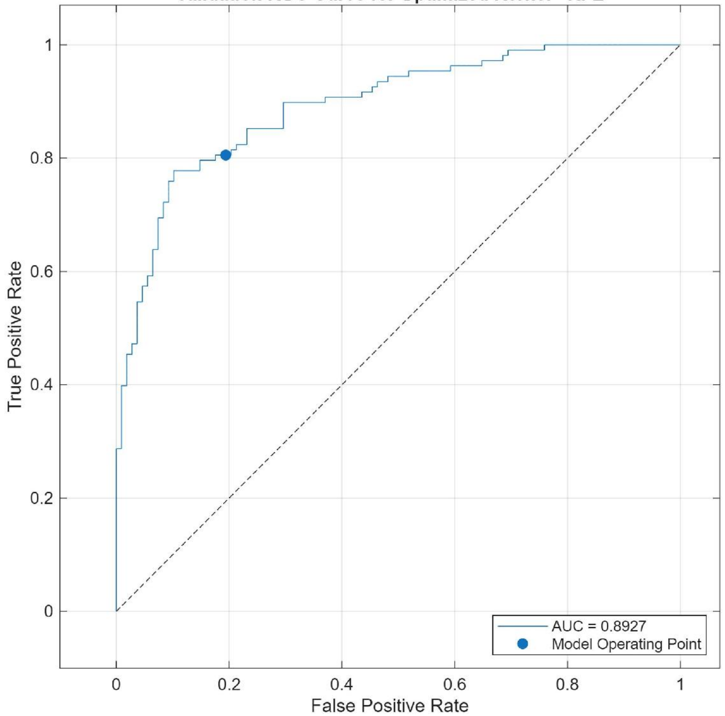
Validation ROC Curve for Optimized Kernel - RFE
