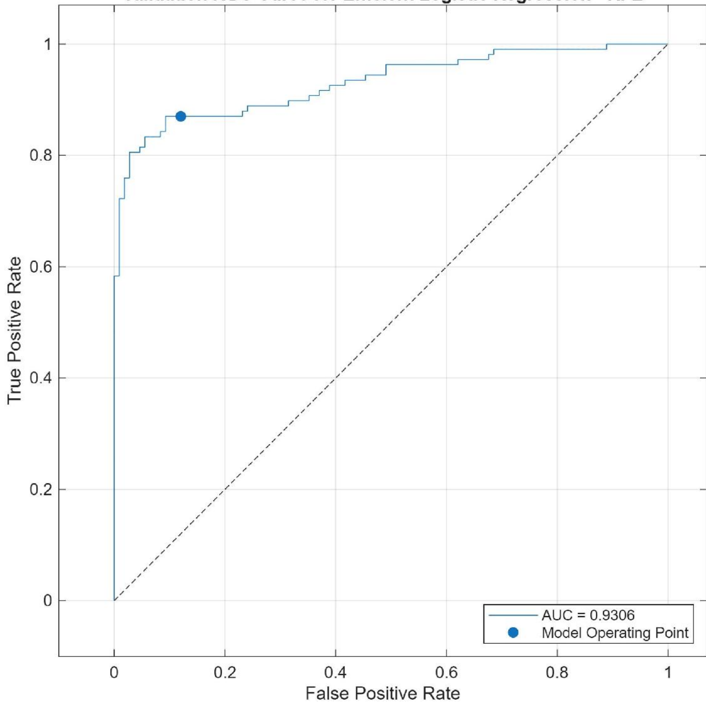
Validation ROC Curve for Efficient Logistic Regression - RFE
