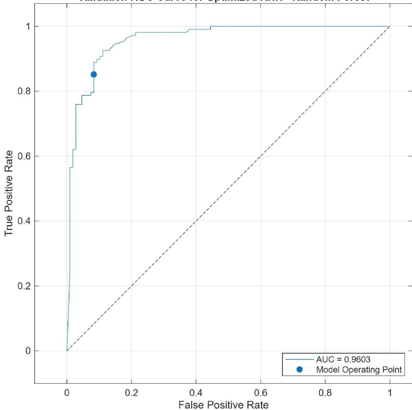
Validation ROC Curve for Optimized KNN - Random Forest
