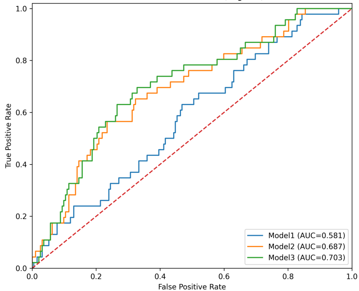
ROC curves on test set (Logistic)
