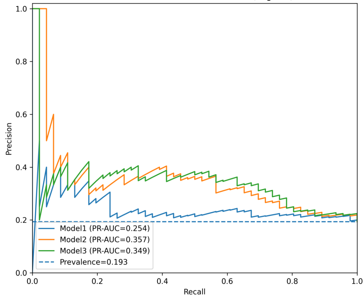
Precision-Recall curves on test set (Logistic)
