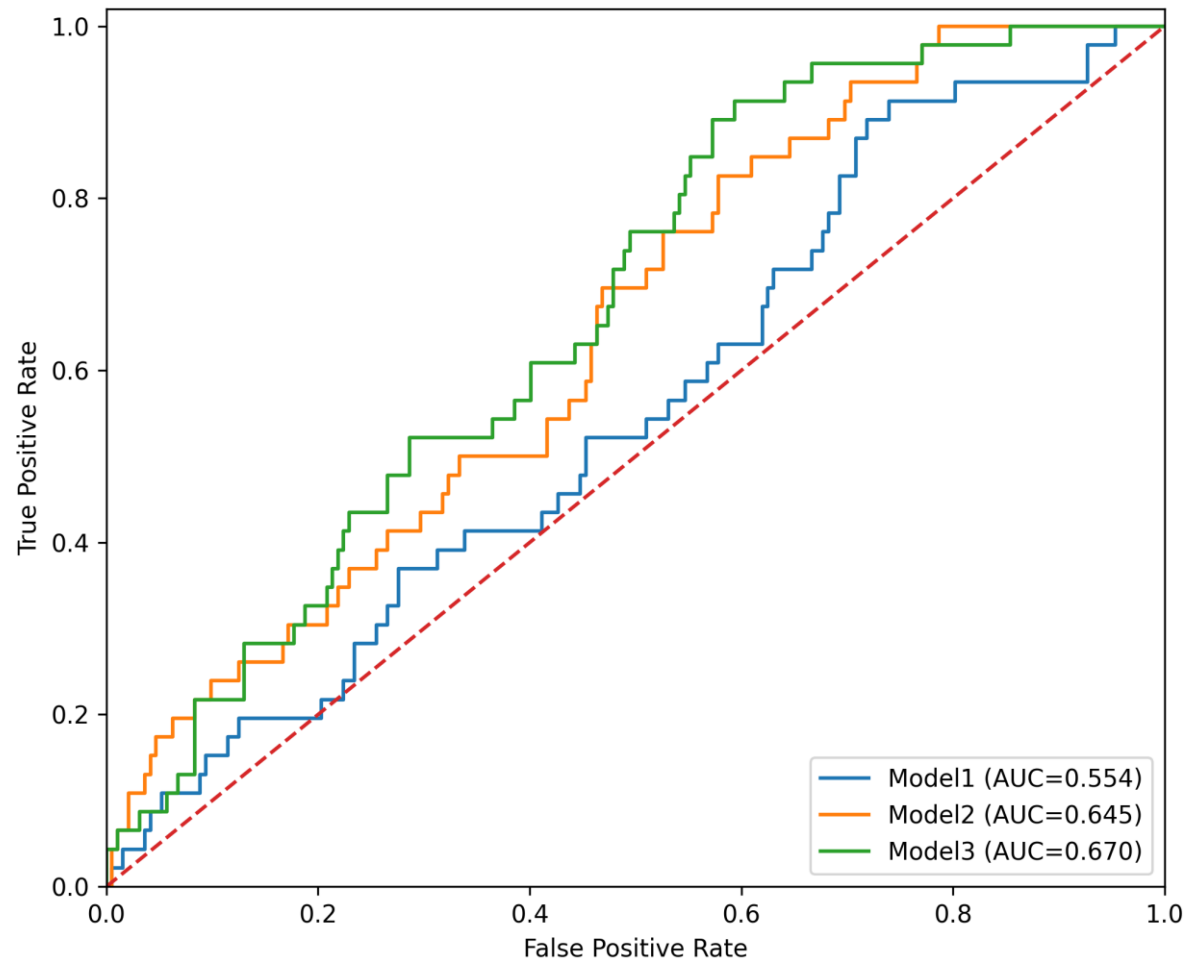
ROC curves on test set (CatBoost)
