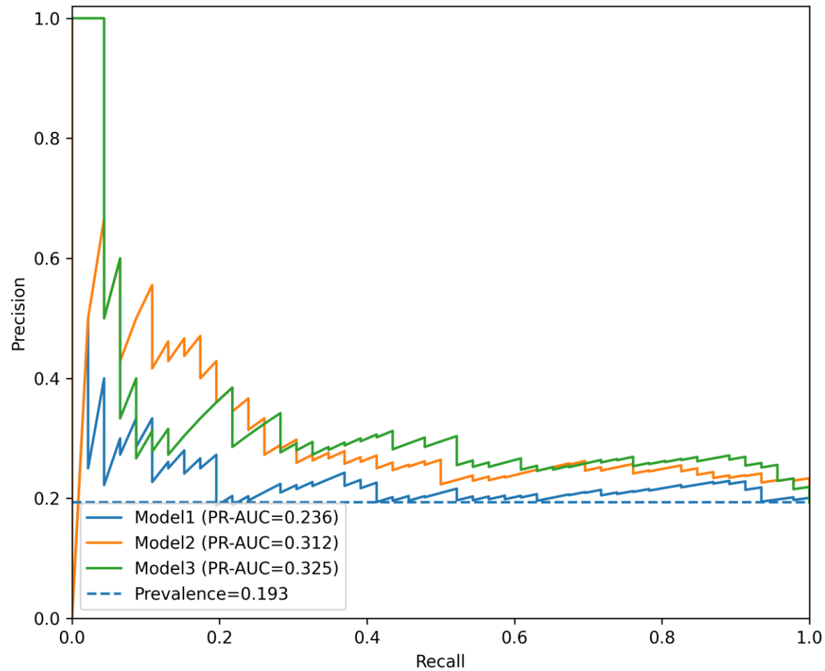
Precision-Recall curves on test set (CatBoost)
