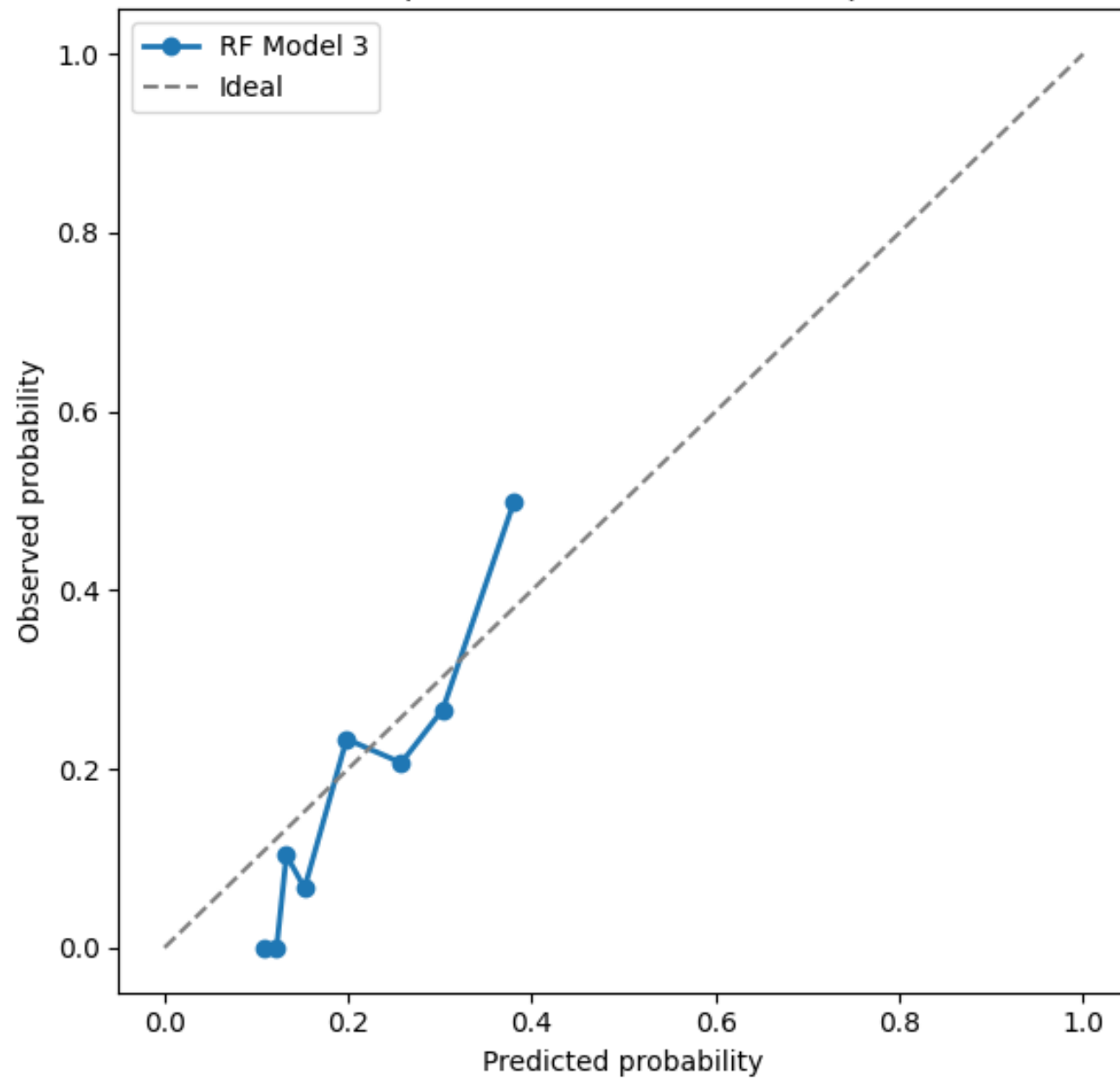
Temporal validation calibration plot
