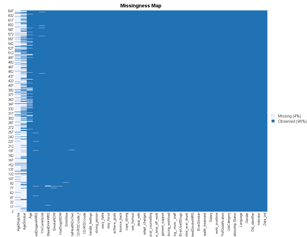
Supplementary Fig. S1: Missingness map of the dataset
