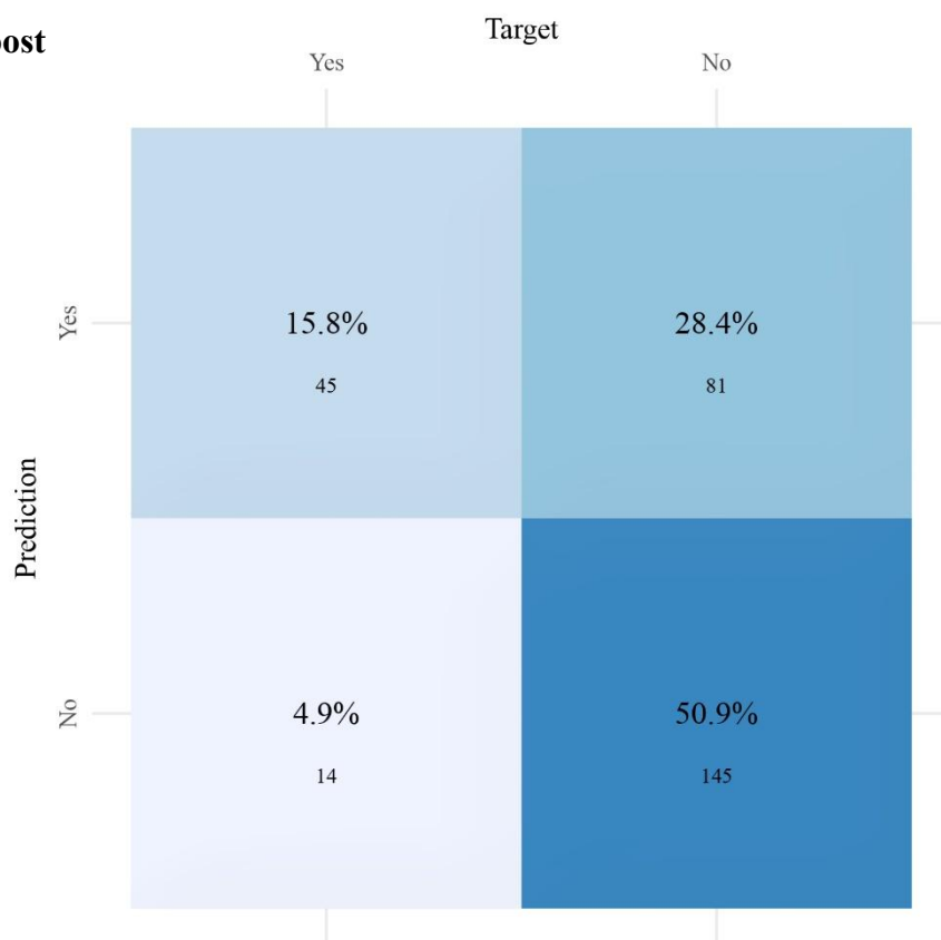
Supplementary figure 1: Confusion matrices of GBM and XGBoost on the test set.
