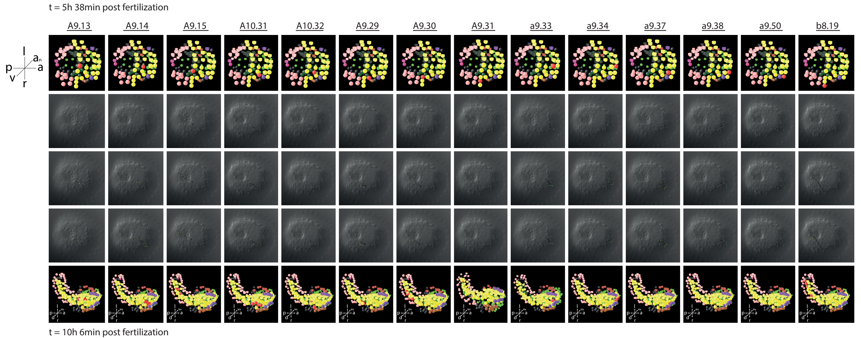
Supplementary Figure 8. Phallusia mammillata . Single cell analysis of nervous system cells at different times of development. Individual cells are marked red in the schematic 3D-representations in the top rows. Rows with Nomarski images show changes in cell position in different numbers of consecutive generations, starting with 1 in the first image of respective column. Schematic 3D-representation in lower row shows descendants of individual cell in the respective column (some descendants might be missing). In all images the trunk of the embryo is oriented as depicted in the axis-orientation labels in the upper left of the figure, unless specified in the respective image.
