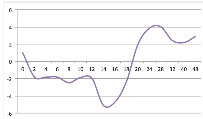
Nvfoxq2-like3 Cp_0hpf: 33.31
