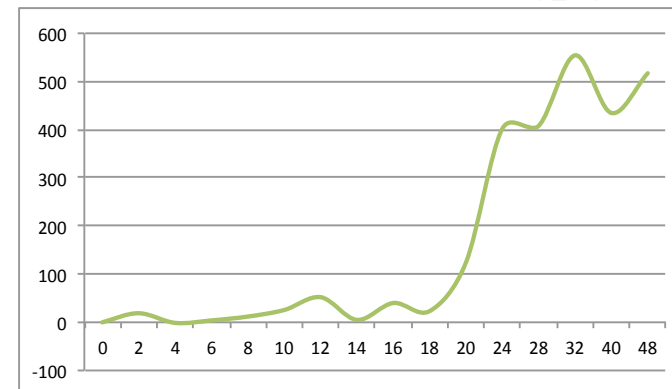
Nvgfi-like Cp_0hpf: 38.94
