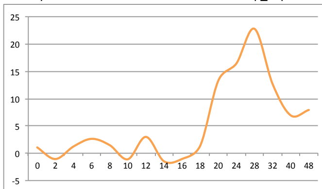
Nvcoup-like2 Cp_0hpf: 33.31
