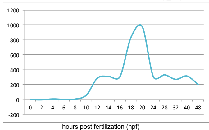
Nvath-like Cp_0hpf: 36.17
