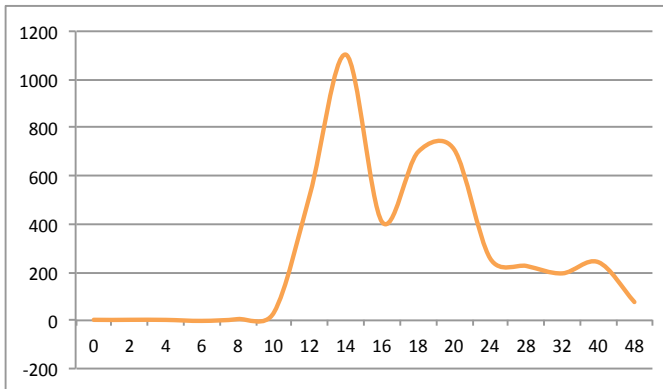
Nvhes3 Cp_0hpf: 35.77
