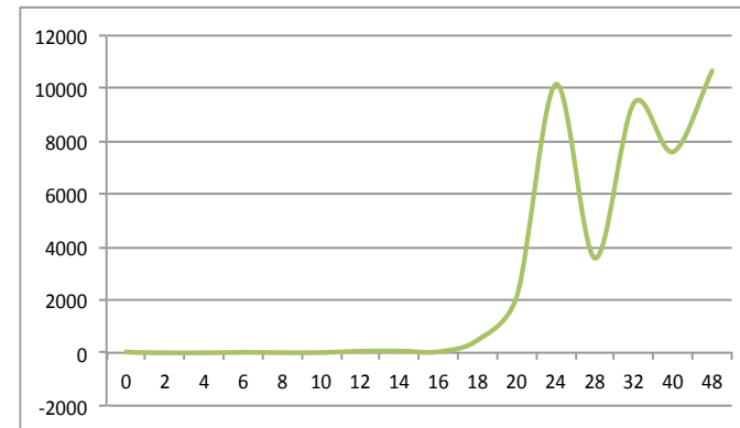
Nvsox2 Cp_0hpf: 40.00
