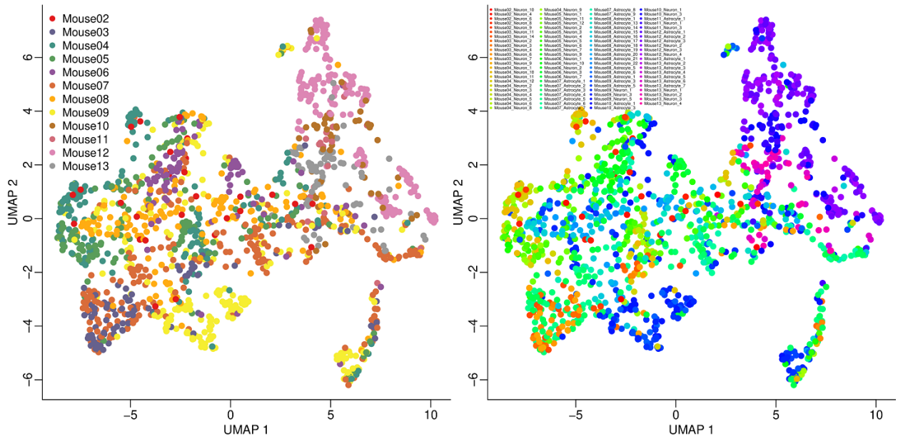
Figure S10. Uniform Manifold Approximation and Projection (UMAP) graph across all single-mitochondria samples.
