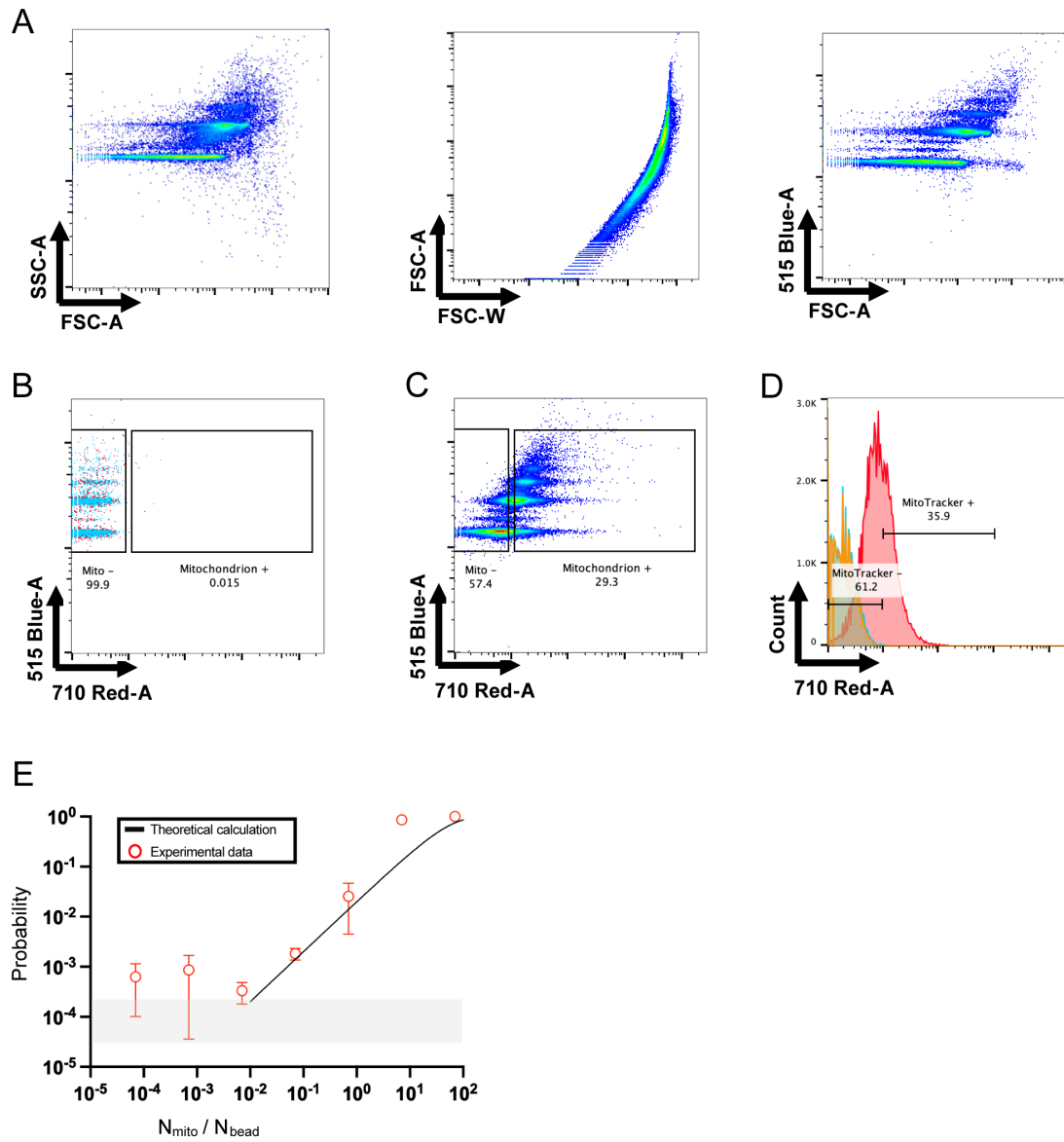
Figure S15. Single mitochondrion isolation from individual neuron or astrocyte cells based on Poisson statistics.
