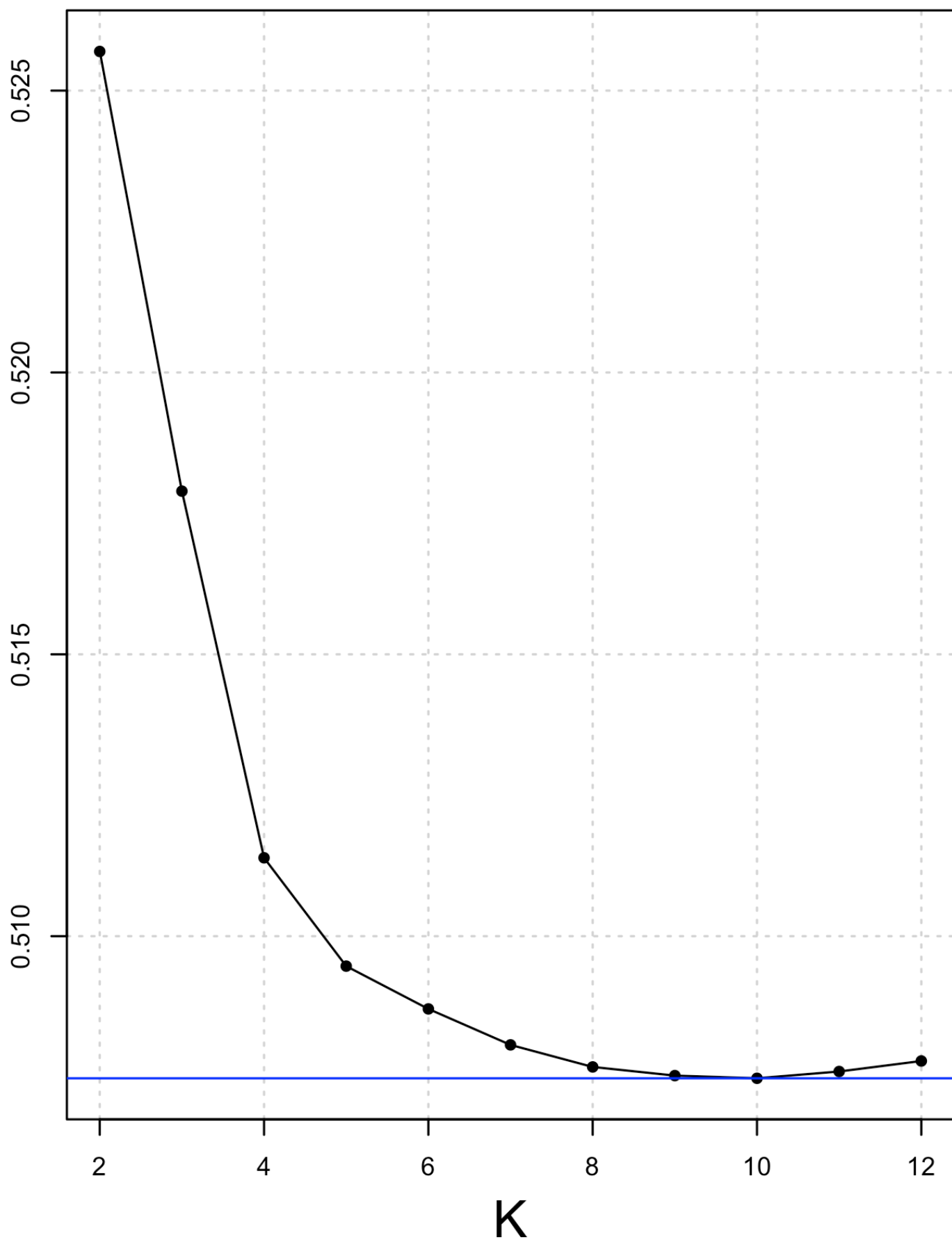
Cross-validation error
