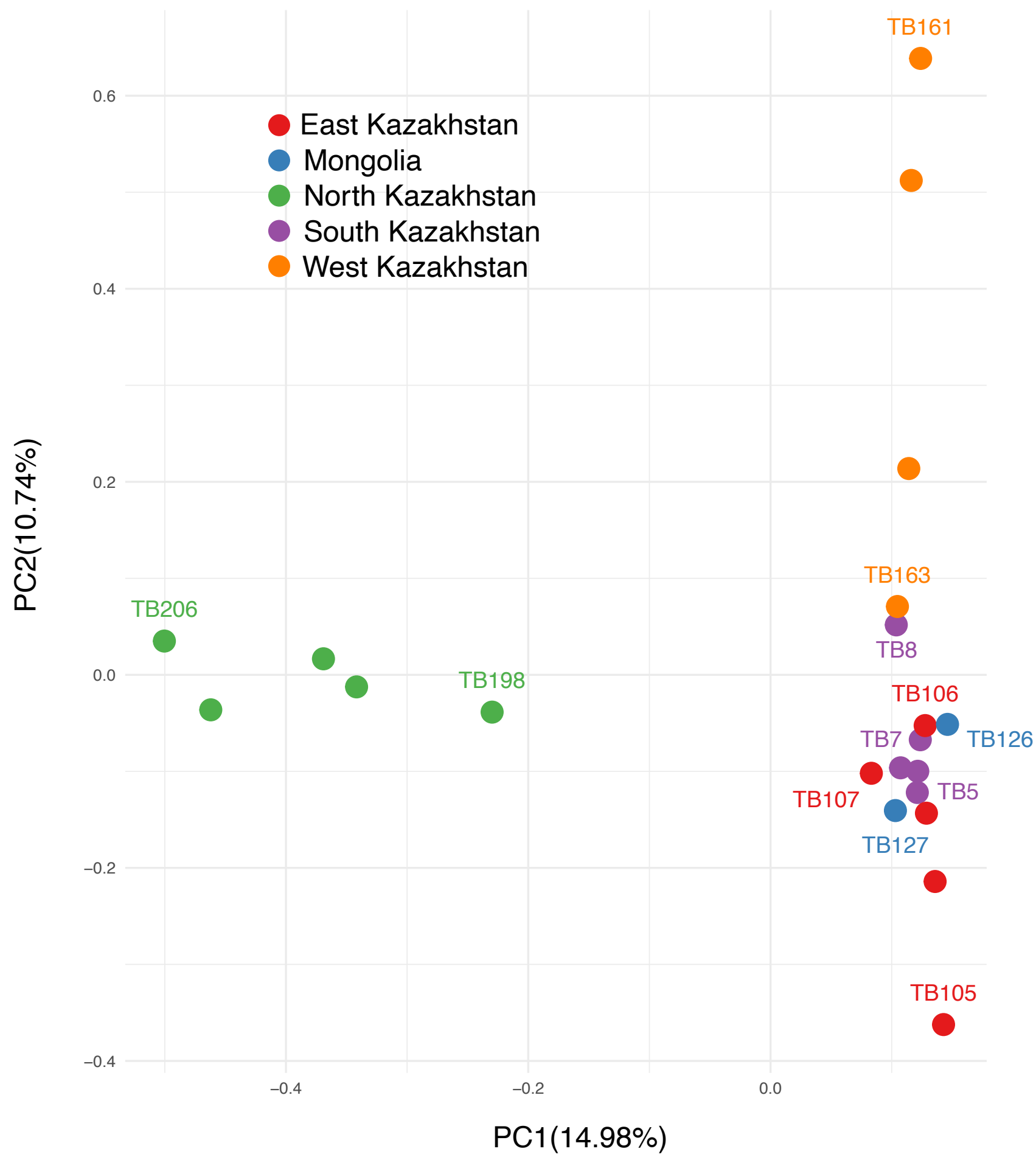
Additional file 2: Fig. S1 Genetic structure of Kazakh Tobet dogs based on a reduced dataset (maximum 5 dogs per region). a PCA plot. b Cross-validation (CV) errors for different K values. c Admixture plot for the best K = 2
