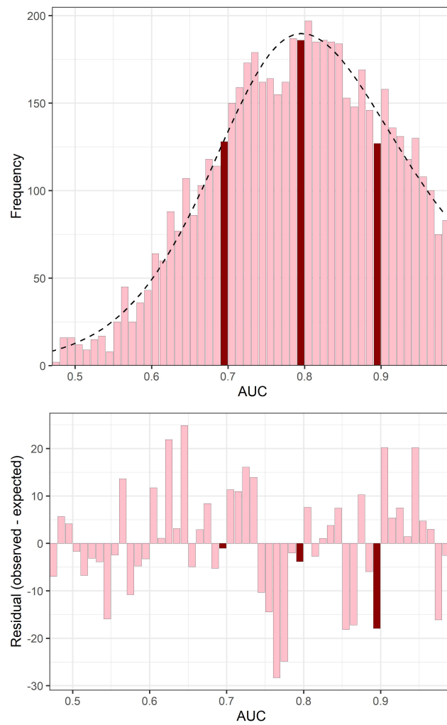
Fig. S5 Subgroup analysis of AUC values from the journal PLOS ONE. Histogram of AUC mean values (top panel) and residuals from a smooth fit to the histogram (bottom panel). The dotted line in the top panel shows the smooth fit.
