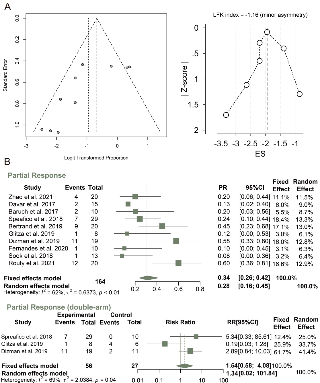
Fig. S3: A: Funnel plot and doi plot with LuisFuruya-Kanamori(LFK) index of studies in partial response (PR) analysis for bias assessment. B: Forest plots of PR rate in all studies and double-arm studies.
