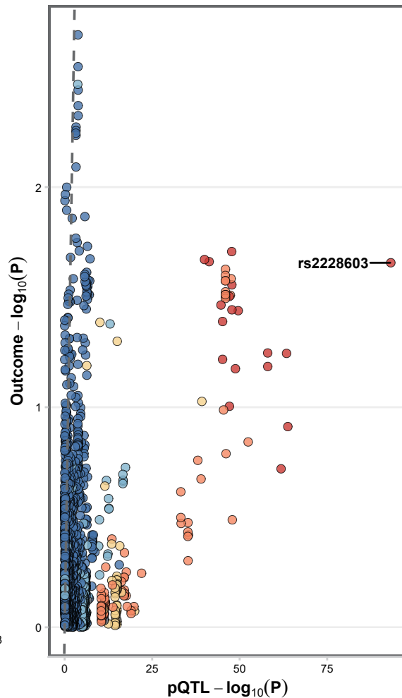
Locus Comparison
