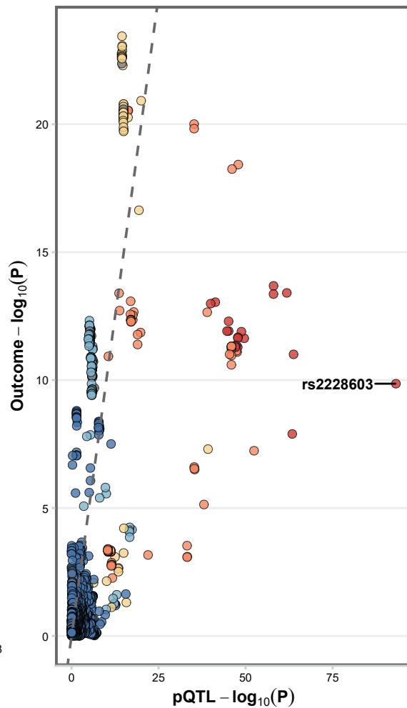
Locus Comparison
