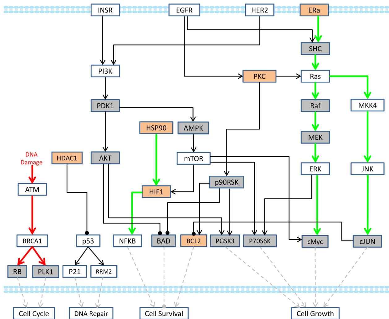
Fig. S5 The response network induced by verapamil. A pathway with red color was up-regulated, green color was down-regulated, black color was un-changed. The edges with yellow color were removed after optimization.
