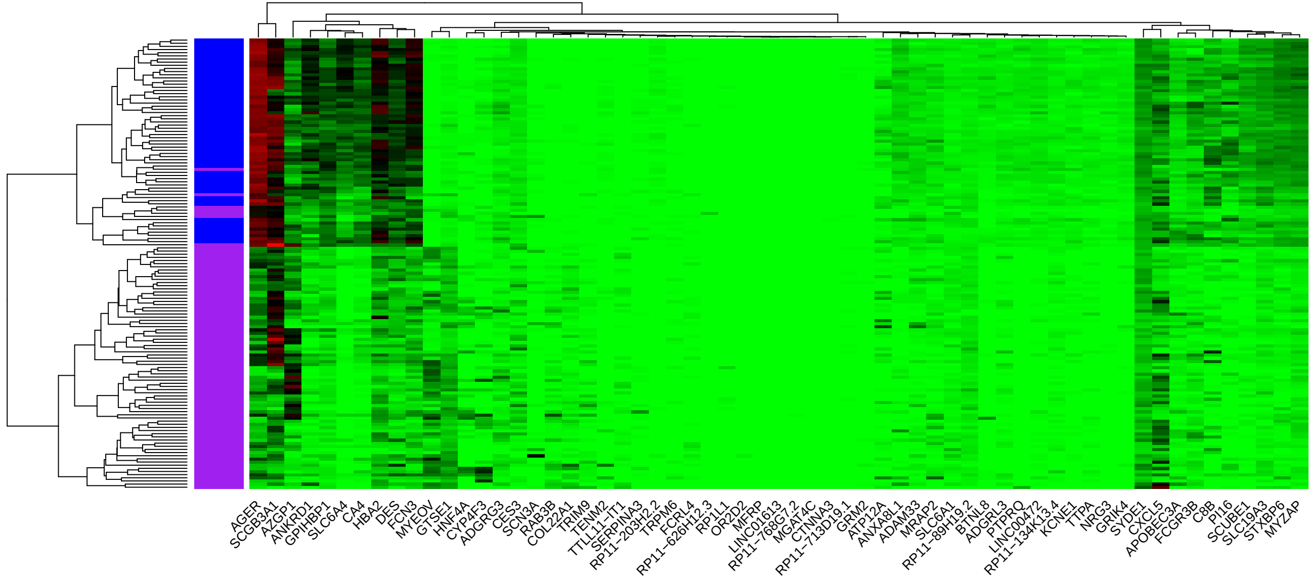
Expression of Normal vs. Stage III
