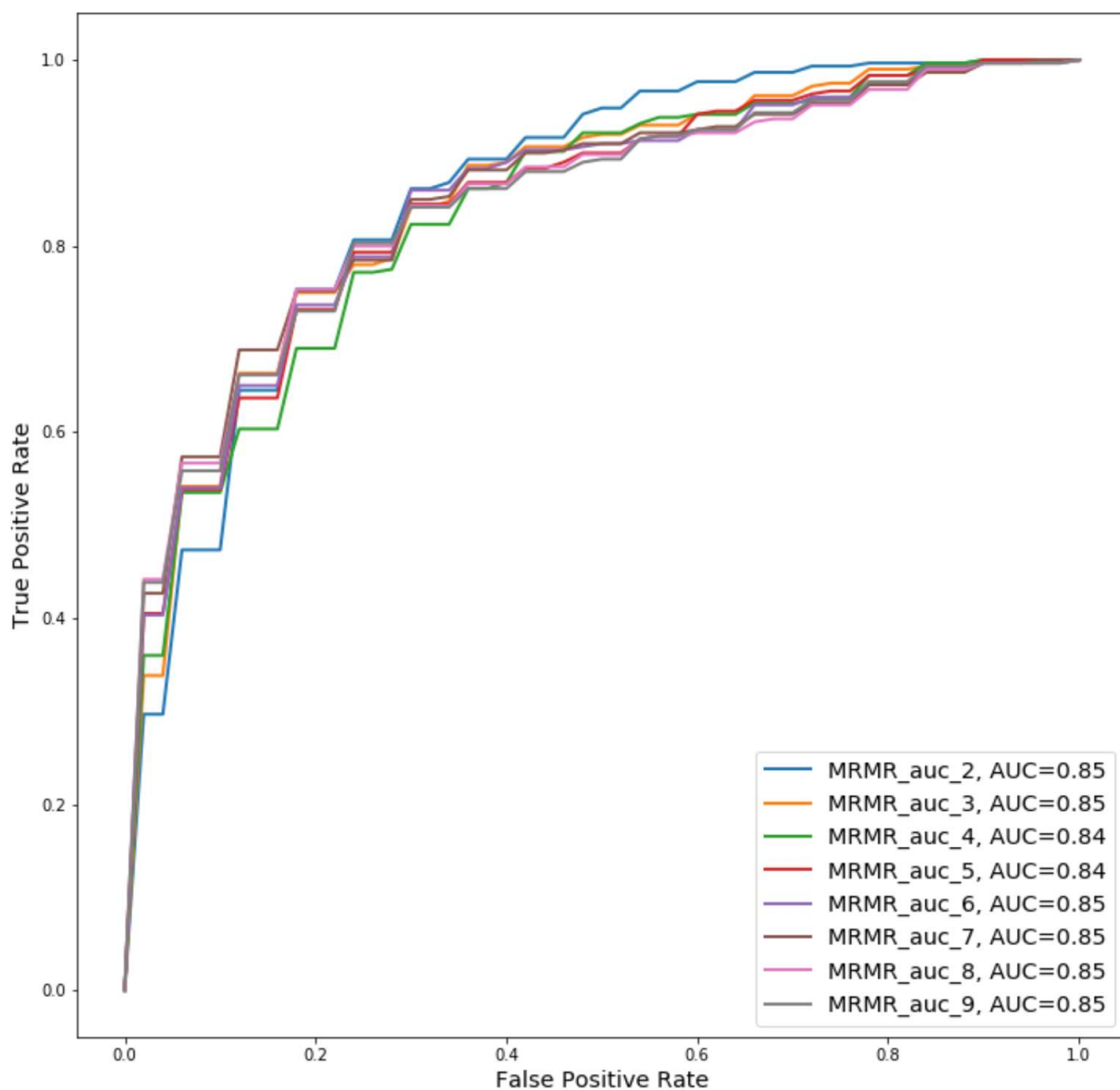
Fig. S3 Average ROC curves of LR models estimated using 10 runs of 10-fold cross-validation and MRMR_auc for selecting top 2,3,...,9 marker genes from the 108 DEGs.
