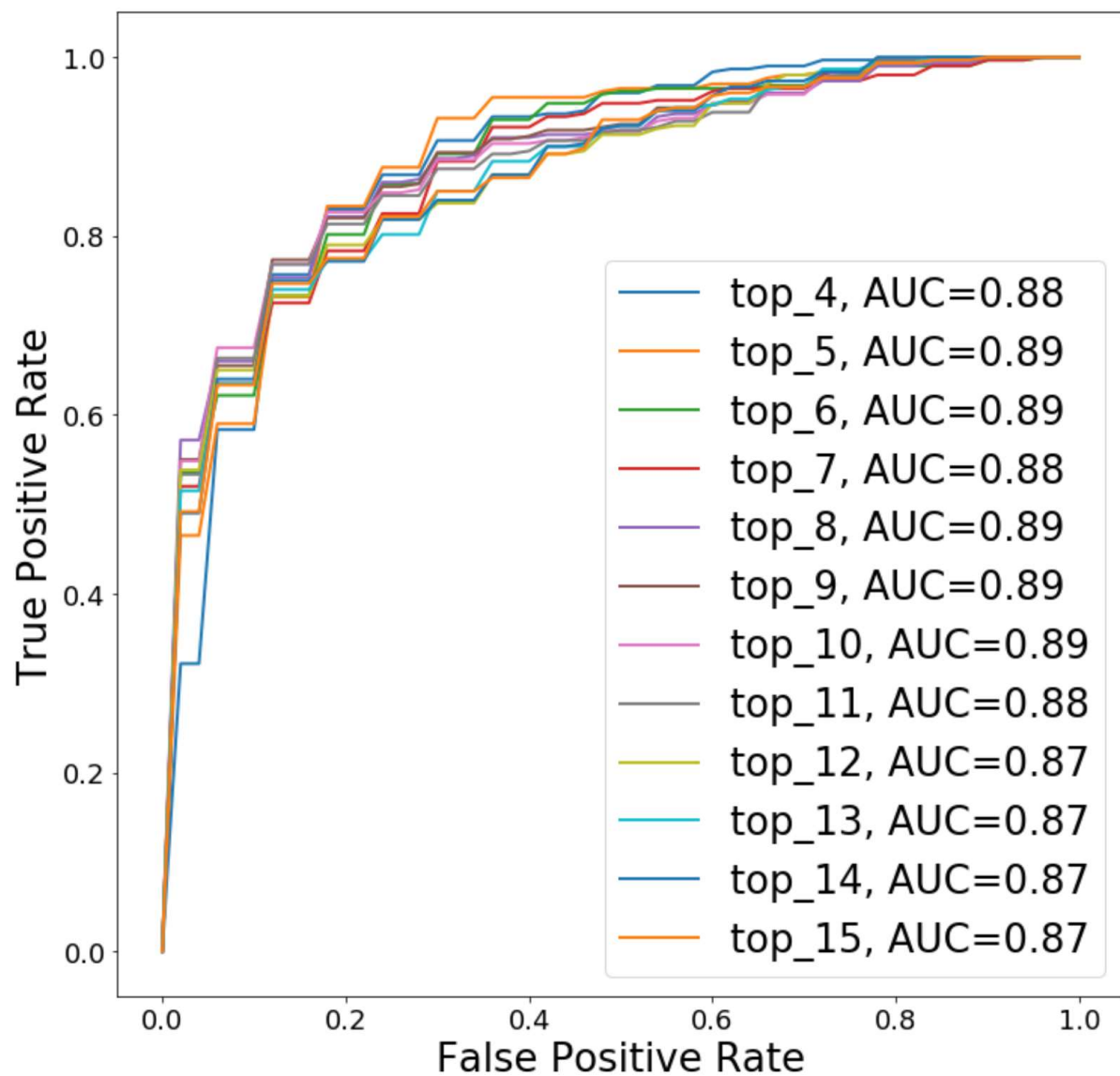
Fig. S4 Average ROC curves of LR models estimated using 10 runs of 10-fold cross-validation and top re-ranked 4,5,...15 marker genes.
