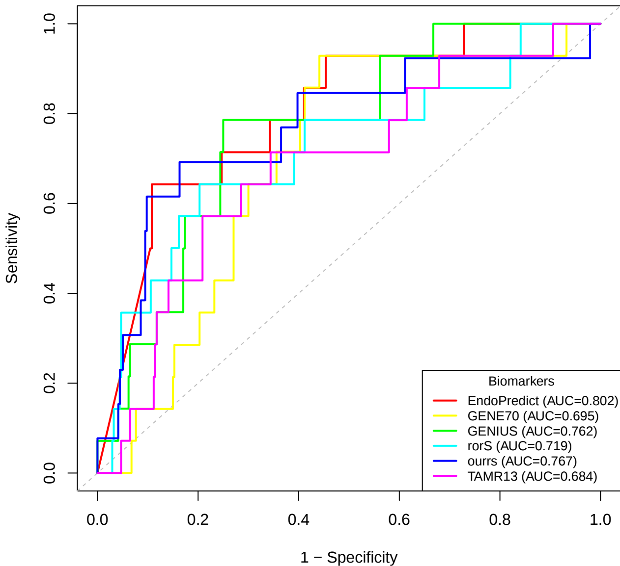
3-Year Overall Survival ROC Curve
