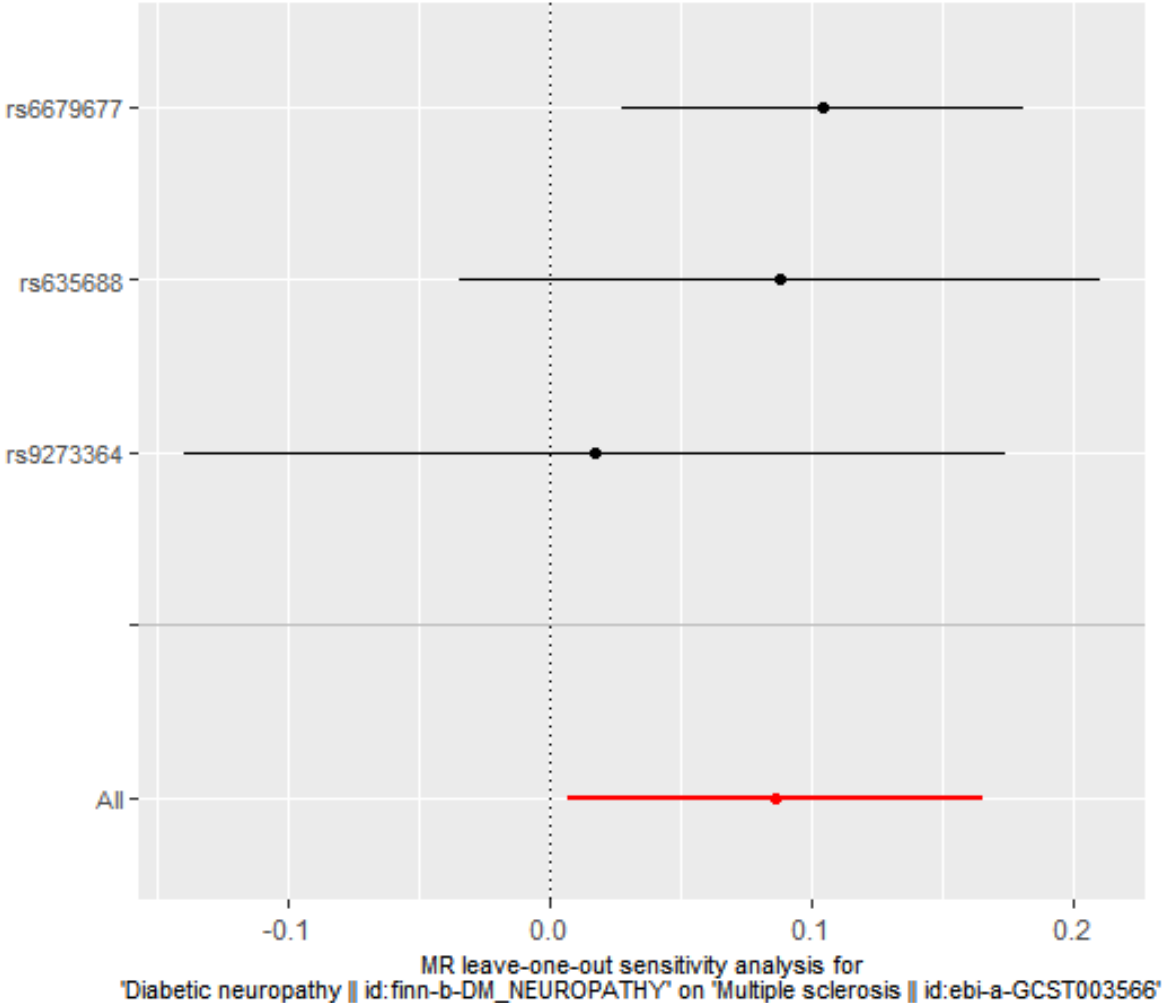
Outcome of the “leave-one-out” sensitivity analysis
