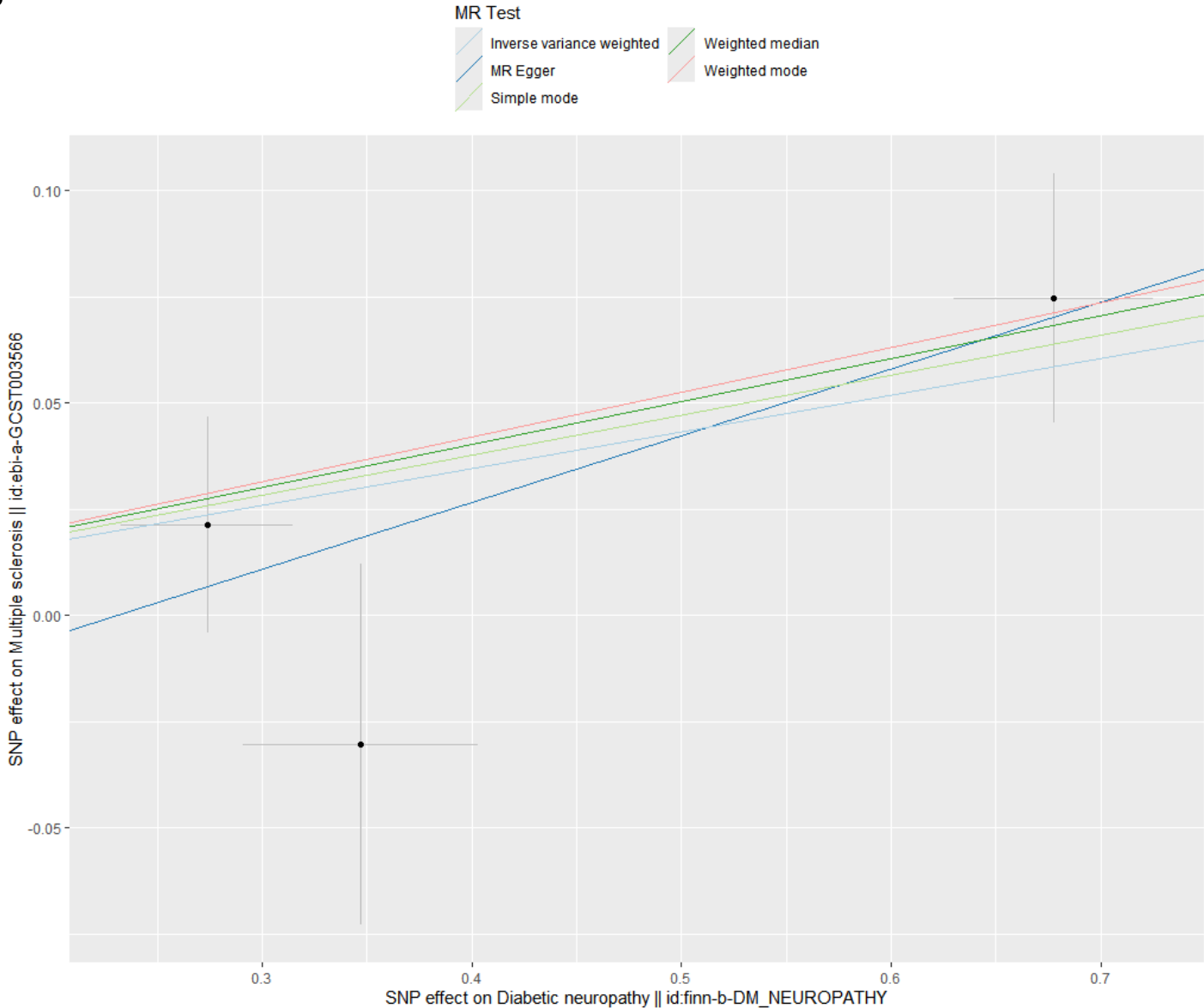
Scatter plot of the two-sample Mendelian randomization analysis
