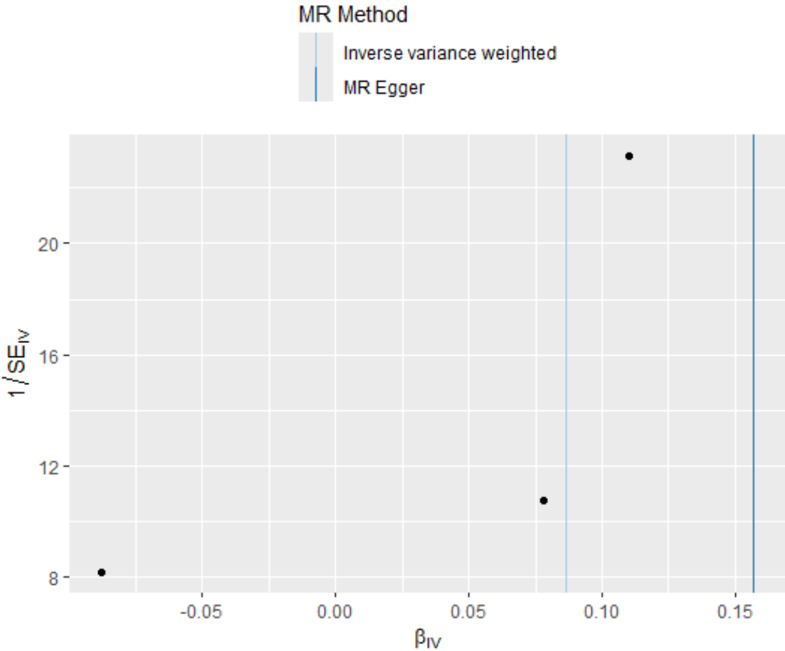
Funnel plot assessing heterogeneity
