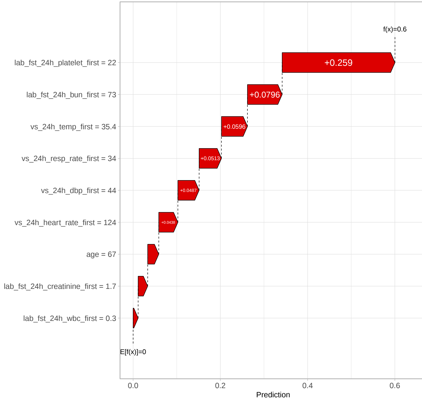
XGBoost – SHAP Waterfall Plot for High-Risk Pneumonia Mortality Patient
