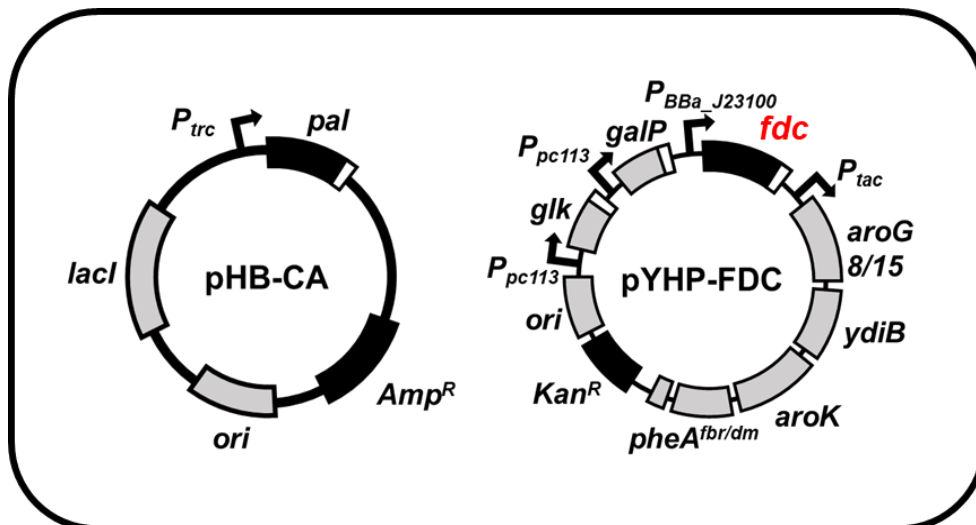
Additional file 1: Figure S1. Schematic diagram of plasmid constructs for the expression of ScFDC gene. (A) E. coli YHP05 harboring pHB-CA-FDC and pYHP. ScFDC gene was cloned in pHB-CA-FDC under the P trc promoter (B) E. coli YHP05 harboring pHB-CA and pYHP-FDC. ScFDC gene was cloned in pYHP-FDC under the constitutive BBa_J23100 promoter.
