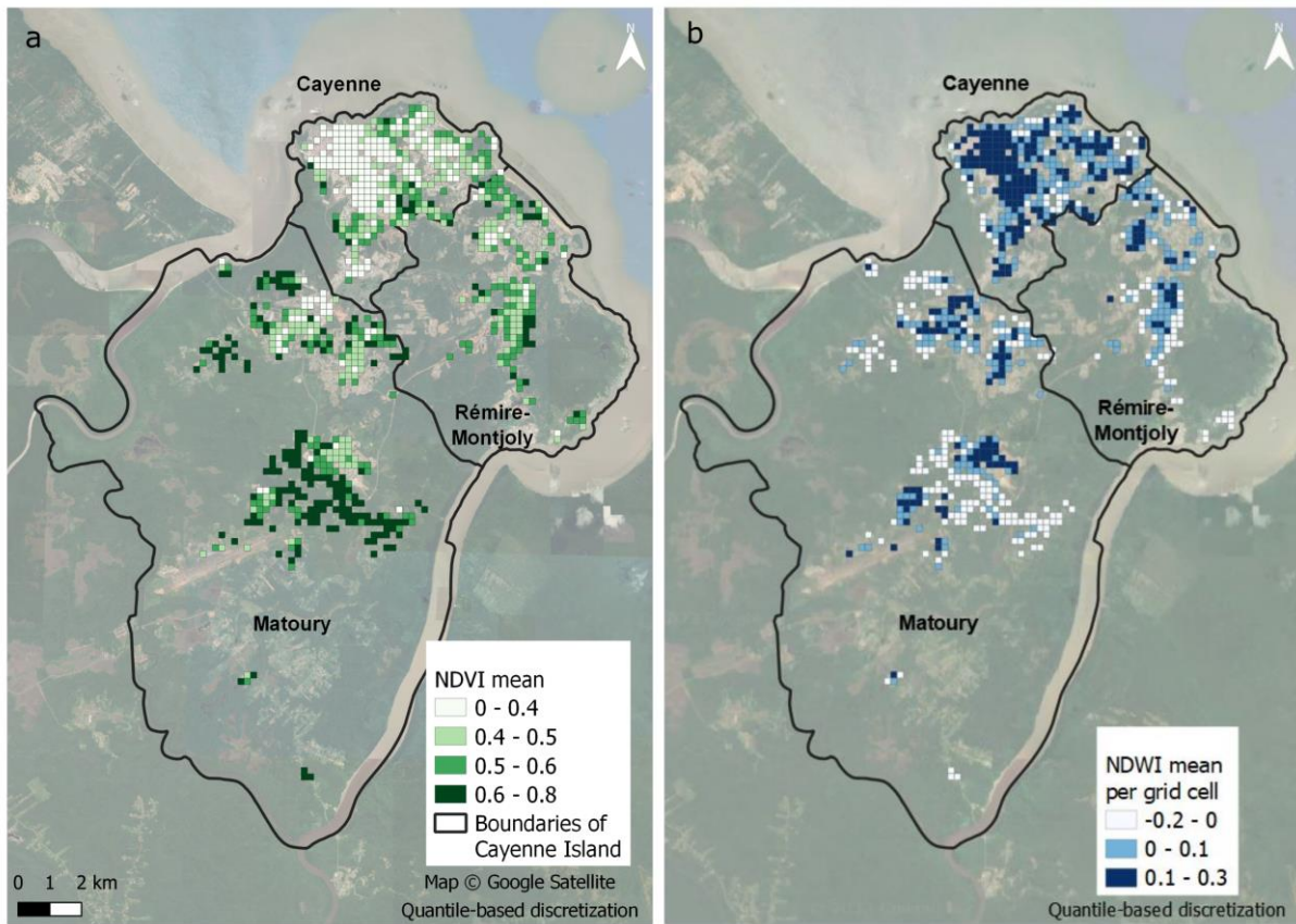
Additional file 2: (a) Mean NDVI on the analysis grid; (b) Mean NDWI on the analysis grid over Cayenne Island.
