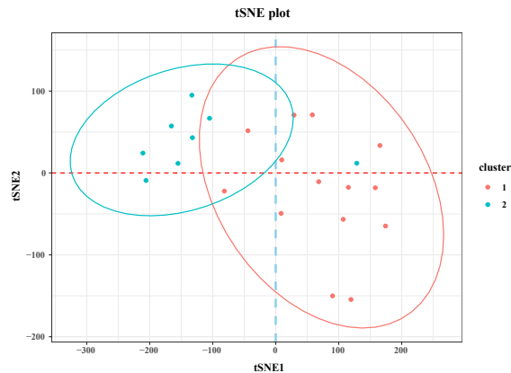
The expression of 19 DEGs in cluster 1 and cluster 2
