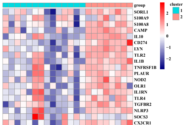
The heatmap of 19 DEGs in cluster 1 and cluster 2
