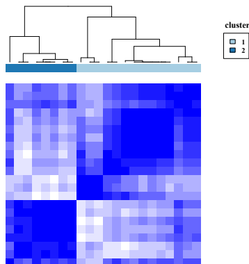
Consensus matrix k=2
