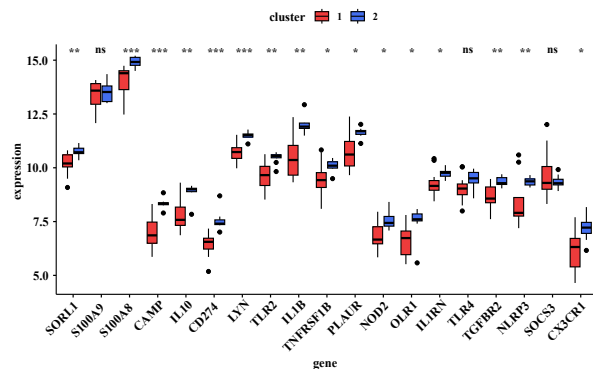
The expression of 19 DEGs in cluster 1 and cluster 2
