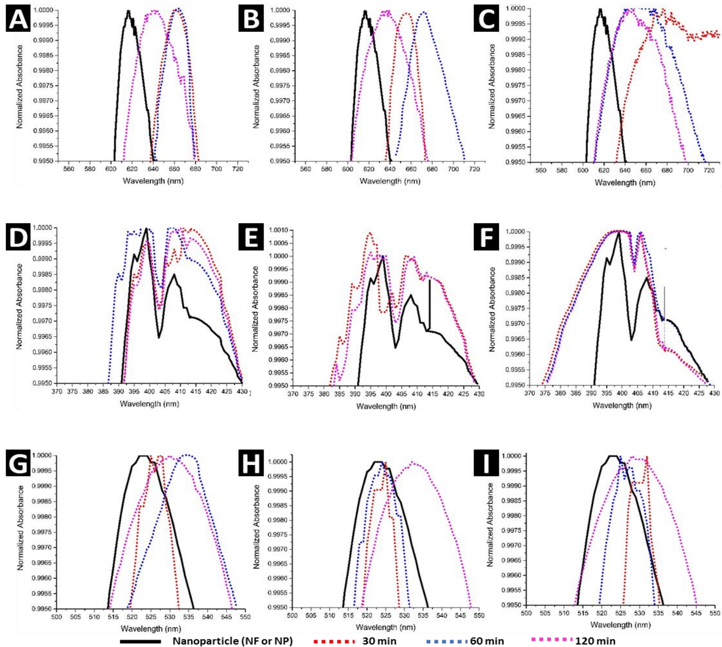
UV-vis analysis to evaluate specificity towards RSV by the functionalized copper (A, B and C) silver (D, E and F) and gold nanoparticles (G, H and I) in presence of Adenovirus (3 replicates).
