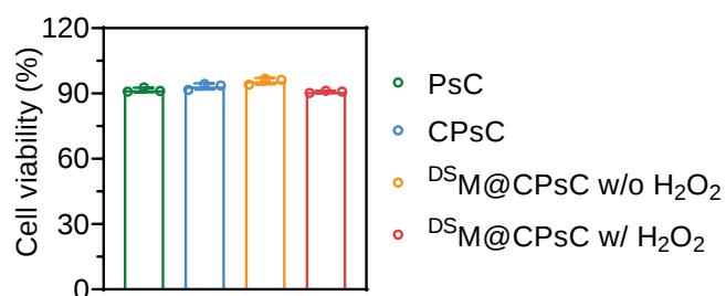
Figure S15. Cytotoxicity of PsC NCs, CPsC NCs, ^{DS}M@CPsC NCs, or H_2O_2 (100 \mu M, 4 h)-pretreated ^{DS}M@CPsC NCs in MSCs following 24-h incubation ( n = 3 ).
