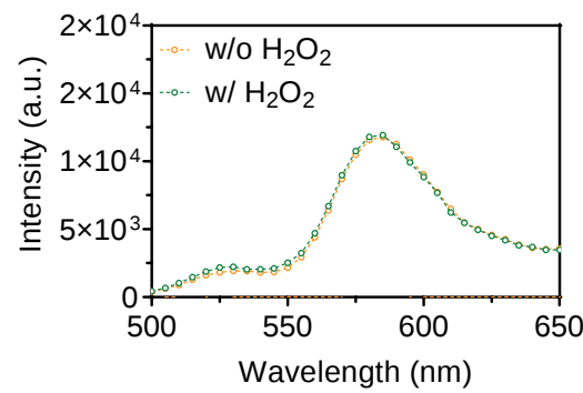
Figure S12. Fluorescence emission spectra ( \lambda_{\text{ex}} = 494 \text{ nm} ) of FAM-siCkip-1-containing DS M@BPSC NCs with (w/) or without (w/o) H 2 O 2 treatment (100 μM, 4 h). MM was pre-stained with DiI.
