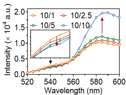
Figure S7. Fluorescence emission spectra ( \lambda_{\text{ex}} = 480 nm) of ^{\text{DS}} M@CPsC NCs composed of DiO-stained MM and Cy3-labeled, DSPE-PEG 2k -conjugated sSDF-1α (Cy3-DS) at various membrane protein/sSDF-1α weight ratios. Black arrow points to the enlarged area.
