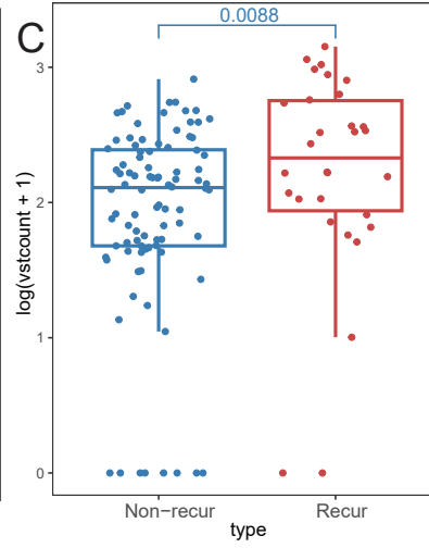
TRIM37
