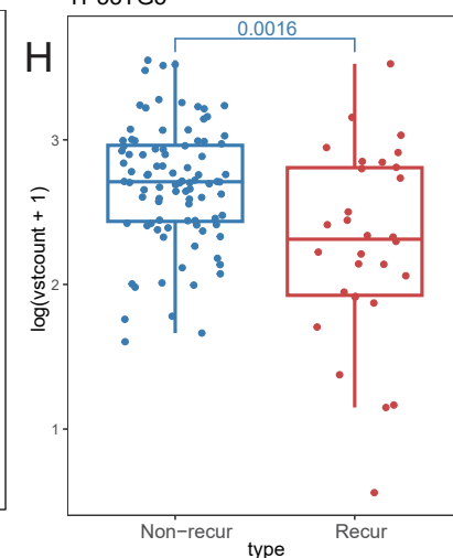
TP53TG5
