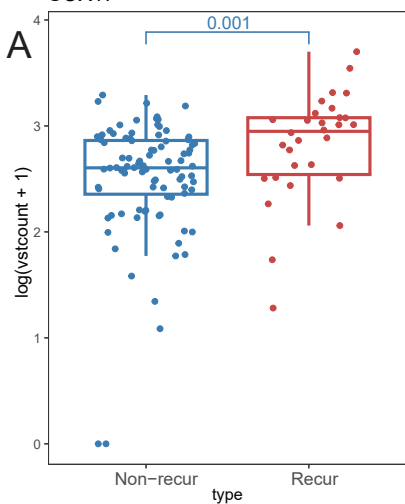
LINC01102
