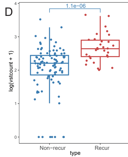
TP53TG5
