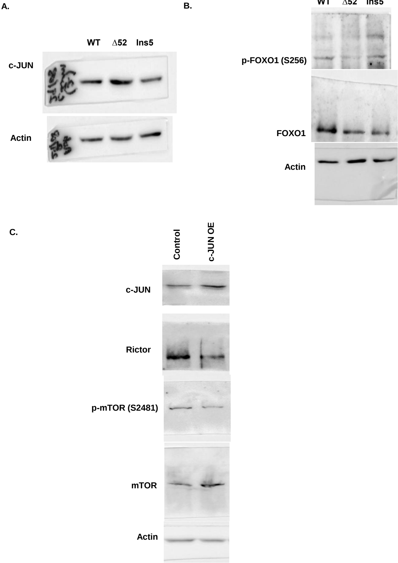
FIGURE 3 A-C
